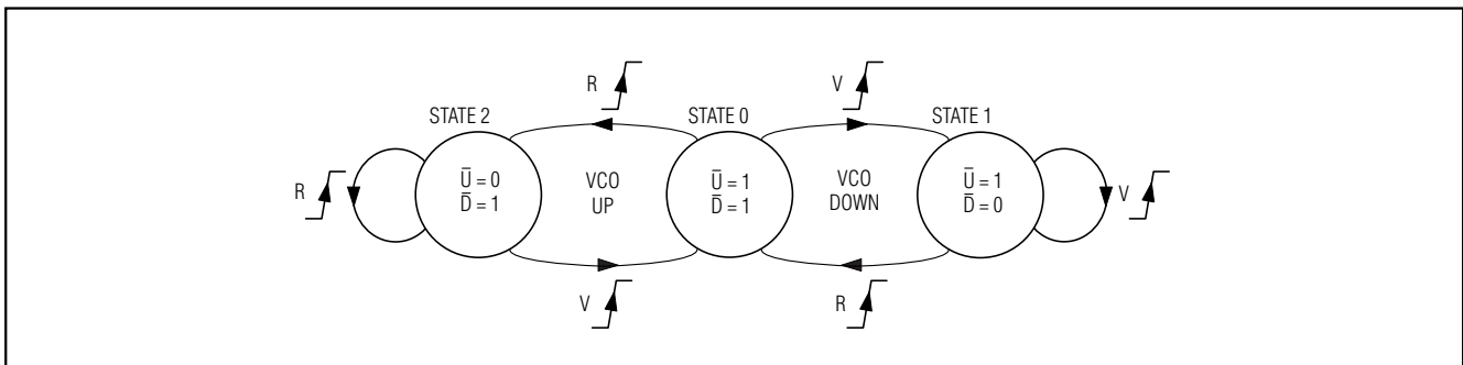
Figure 4. MAX9382/MAX9383 State Diagram
