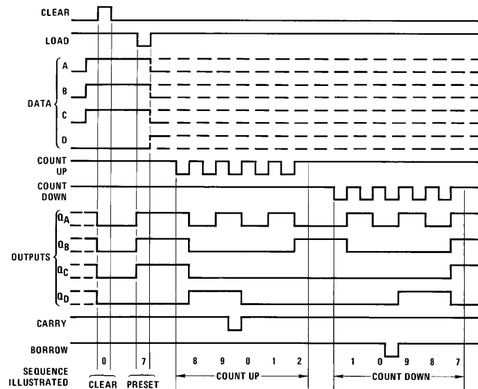
CD40192BM/CD40192BC
