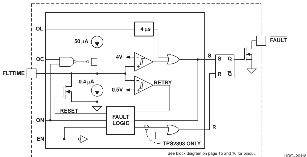
Figure 27. Fault Timer Block Operation
