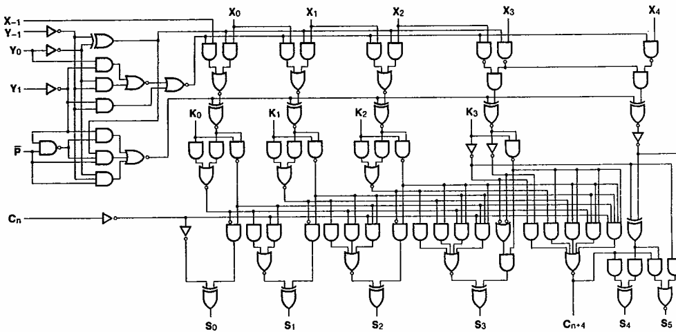
LOGIC DIAGRAM
