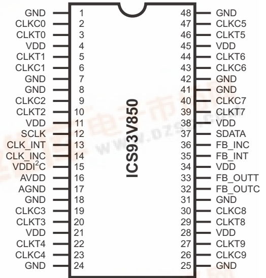
48-Pin TSSOP
