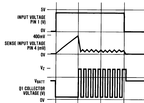
FIGURE 6. Switching Waveforms
