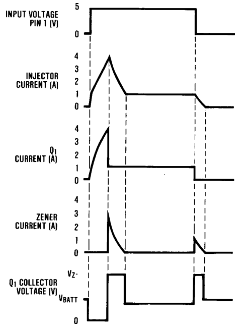
FIGURE 4. Circuit Waveforms
