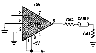
Double Terminated Cable Driver
