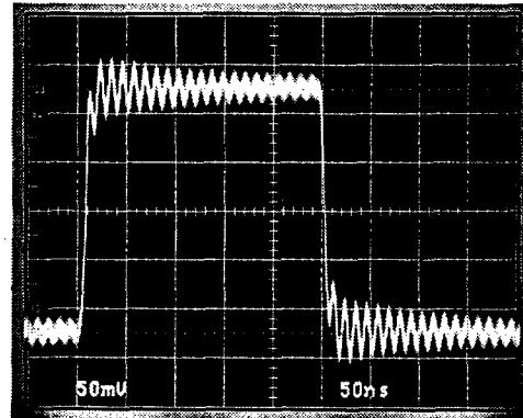
LT1194 IN DEMO BOARD, C_L = 50pF
