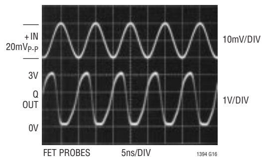
Response to 100MHz ±10mV Sine Wave
