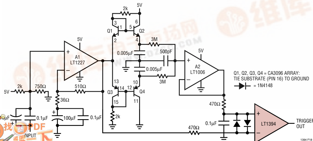
45MHz Single Supply Adaptive Trigger
