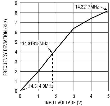
Figure 21. Control Voltage vs Output Frequency for Figure 15. Tuning Deviation from Center Frequency Exceeds ±240ppm
