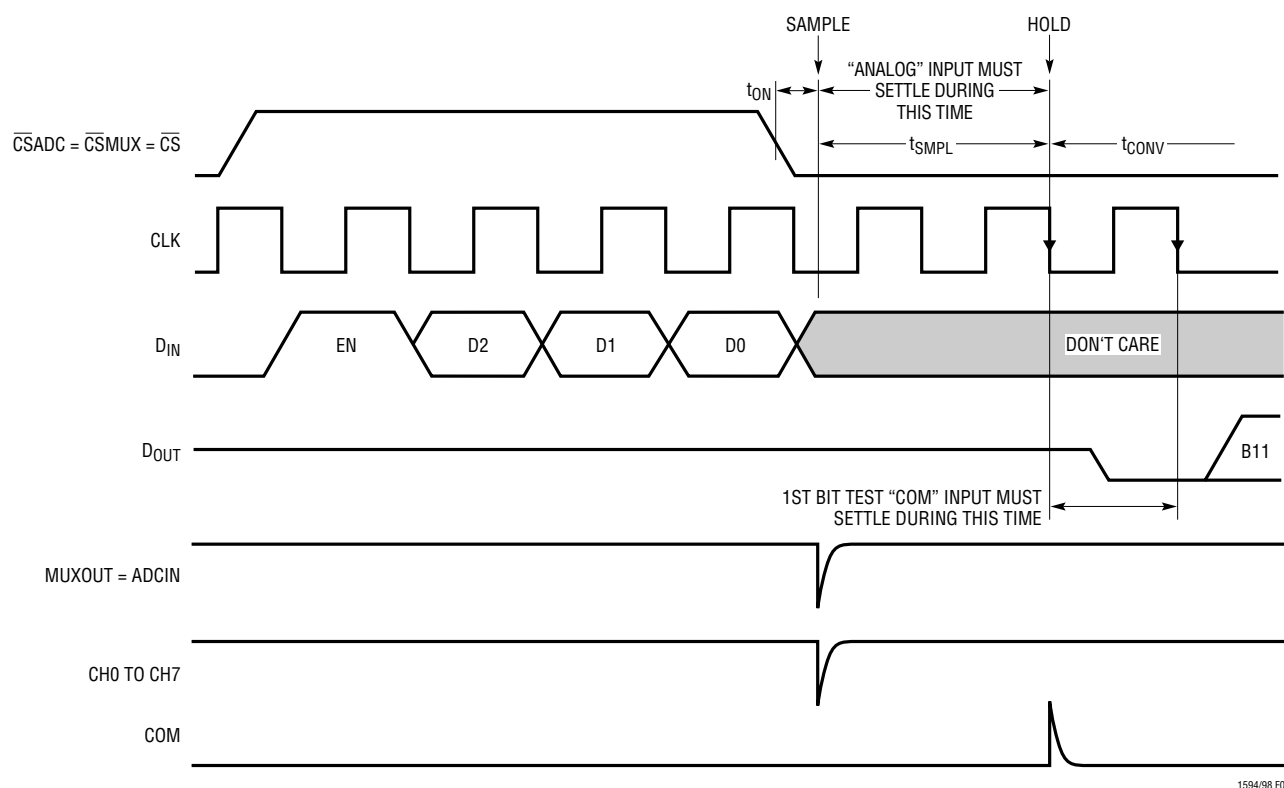
Figure 7. LTC1594/LTC1598 ADCIN and COM Input Settling Windows
