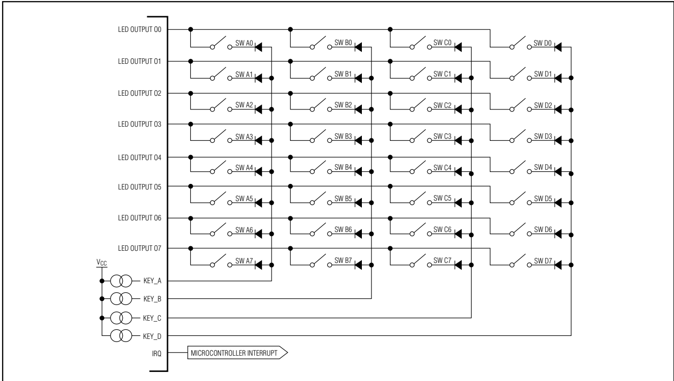
Figure 11. Key-Scanning Configuration
