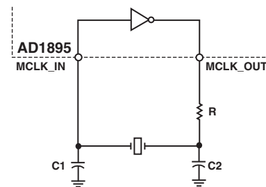
Figure 9a. Fundamental Mode Circuit Configuration
