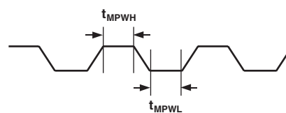
Figure 3. MCLK_IN Timing
