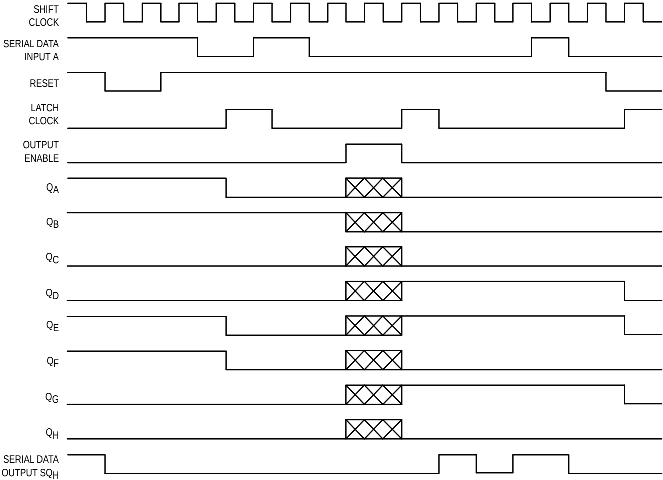
TIMING DIAGRAM
