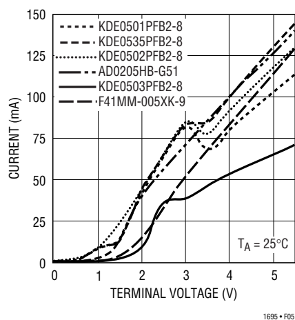
Figure 5. I-V Characteristics of 5V Brushless DC Fan Samples
