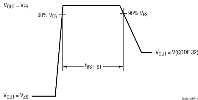
Boost Start Timer Measurement I_{LOAD} = 10\text{mA} , C_{LOAD} = 4.7\mu\text{F}
