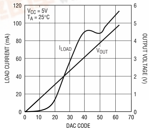
Fan Voltage and Current vs DAC Code
