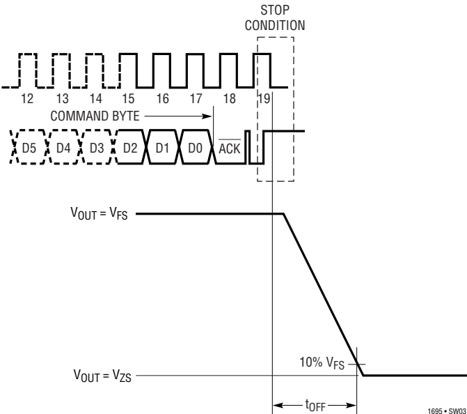
Output Switch Off Time Measurement Code = 0, I_{LOAD} = 150\text{mA} , C_{LOAD} = 4.7\mu\text{F} f_{SMBus} = 100\text{kHz}
