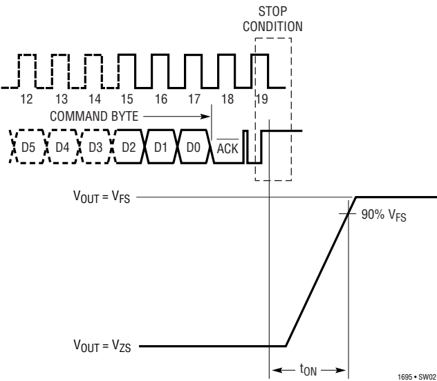
Output Switch On Time Measurement Code = 63, I_{LOAD} = 1\text{mA} , C_{LOAD} = 4.7\mu\text{F} f_{SMBus} = 100\text{kHz}
