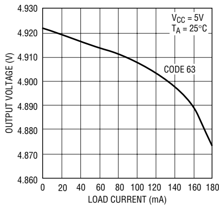
Output Voltage (Full Scale) vs Load Current
