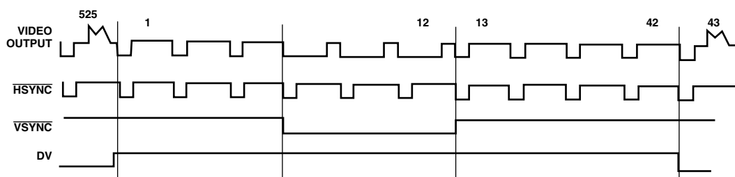
Figure 49. DV Input Control Signal in Relation to Video Output Signal
