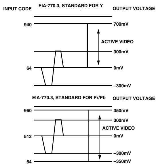
Figure 63. EIA-770.3 Standard Output Signals (1080i, 720p)
