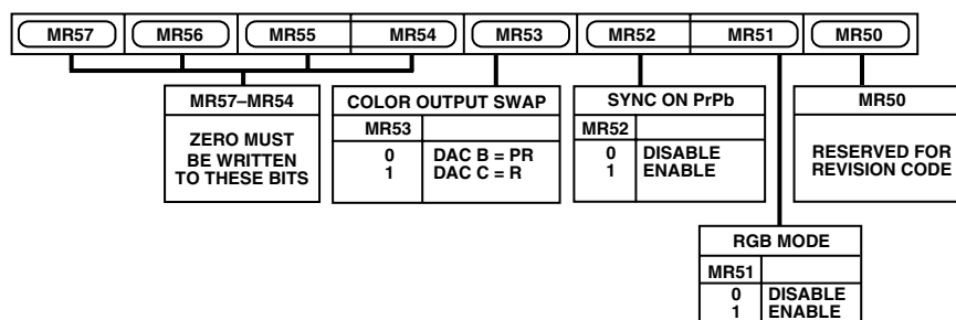
Figure 56. Mode Register 5
