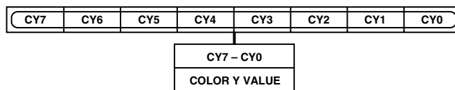
Figure 26. Color Y Register
