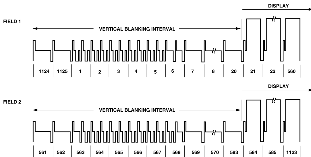
Figure 70. SMPTE274M (1080i)
