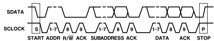
Figure 12. Bus Data Transfer
