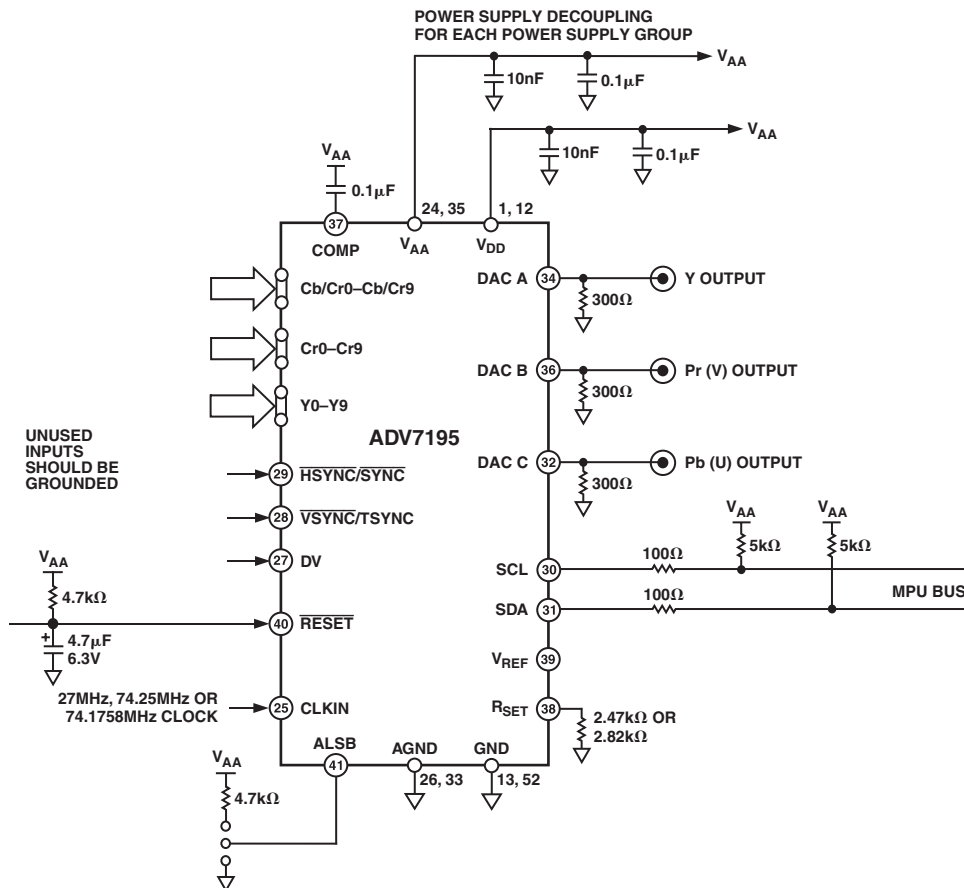
Figure 57. Circuit Layout
