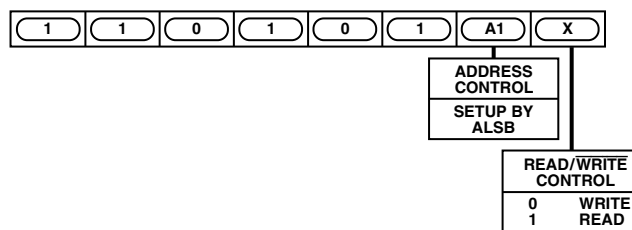
Figure 11. Slave Address
