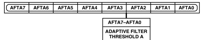
Figure 41. Adaptive Filter Threshold A Register
