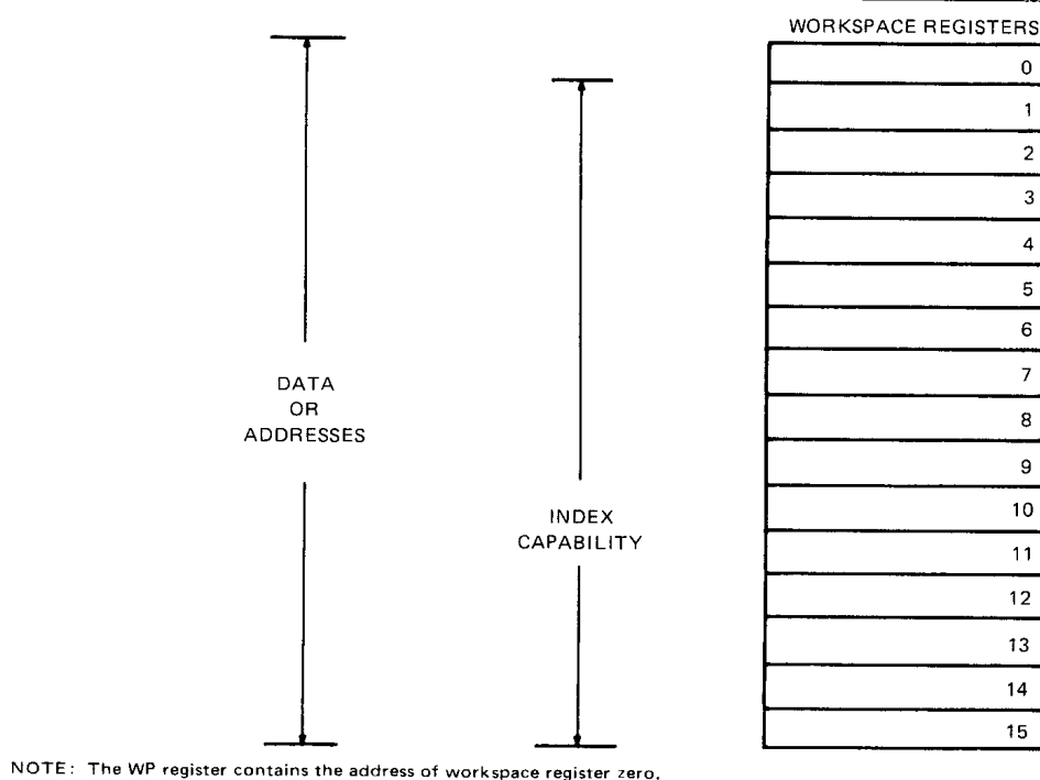
FIGURE 6 – WORKSPACE REGISTERS USABLE AS INDEX REGISTERS
