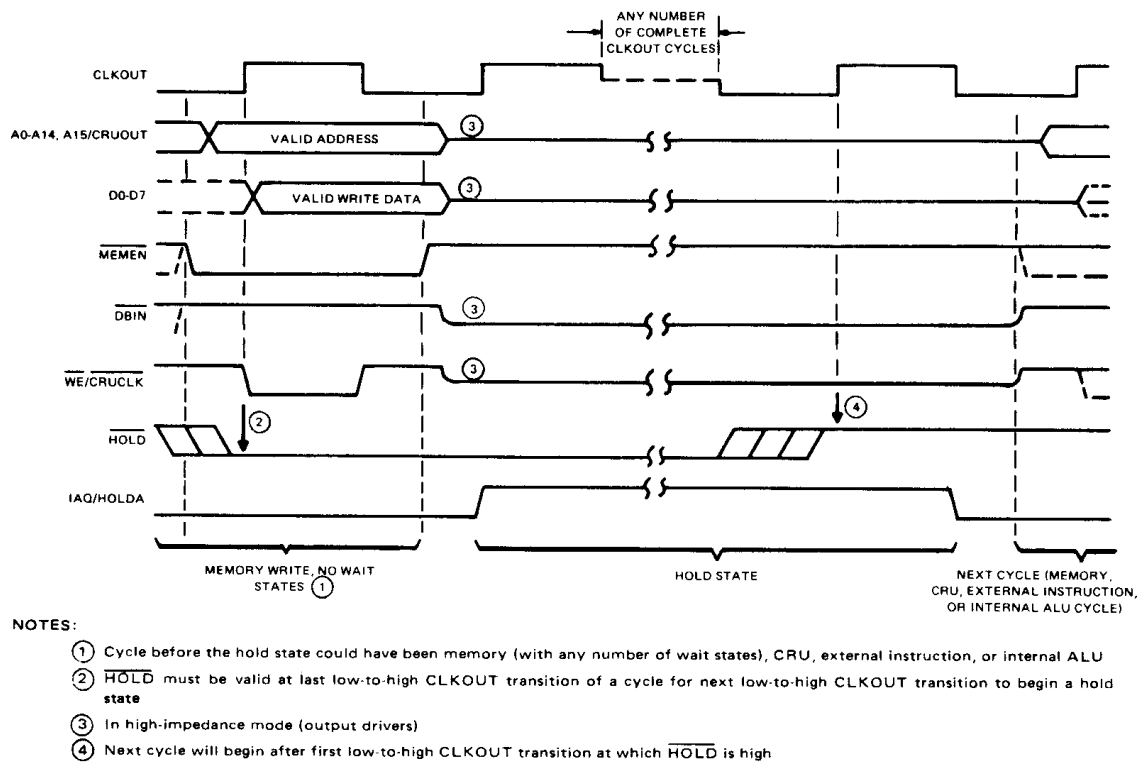
FIGURE 11 – TMS9995 HOLD STATE
