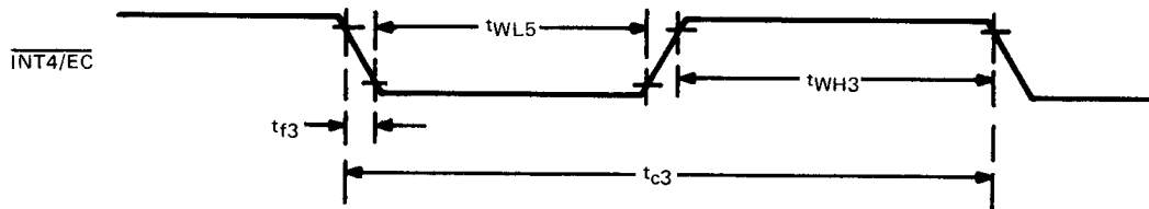
FIGURE 32 – TMS 9995 INTERRUPT INPUT TIMING
