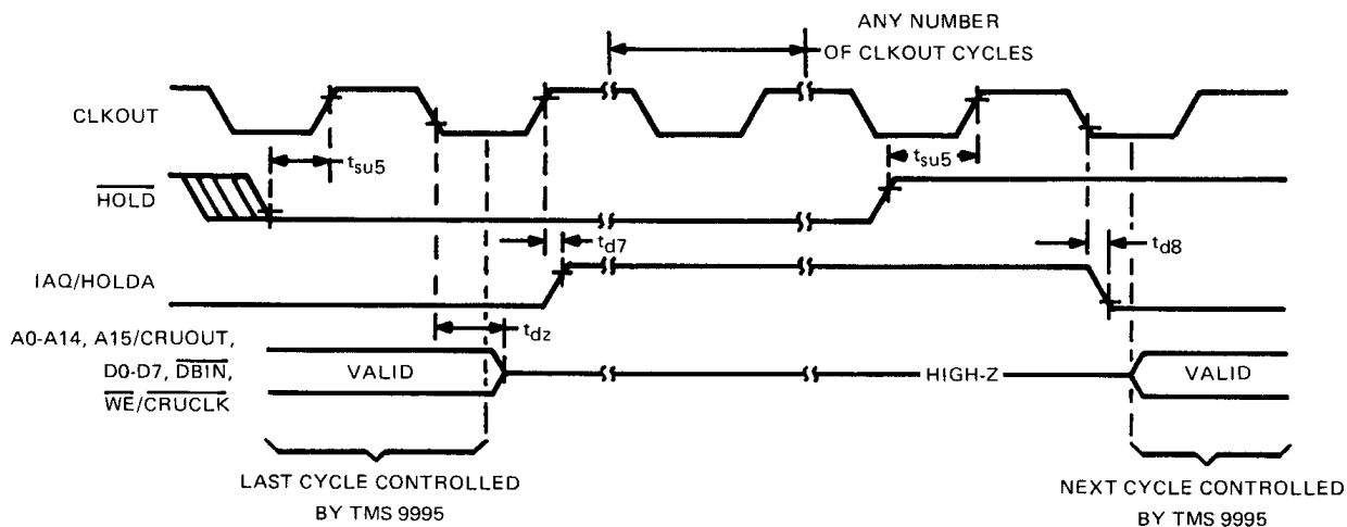
FIGURE 31 – TMS 9995 \overline{\text{HOLD}} TIMING
