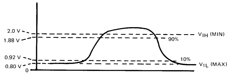
FIGURE 34 – MEASUREMENT POINTS FOR SWITCHING CHARACTERISTICS
