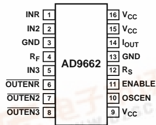
Figure 2. QSO-P16 Pinout
