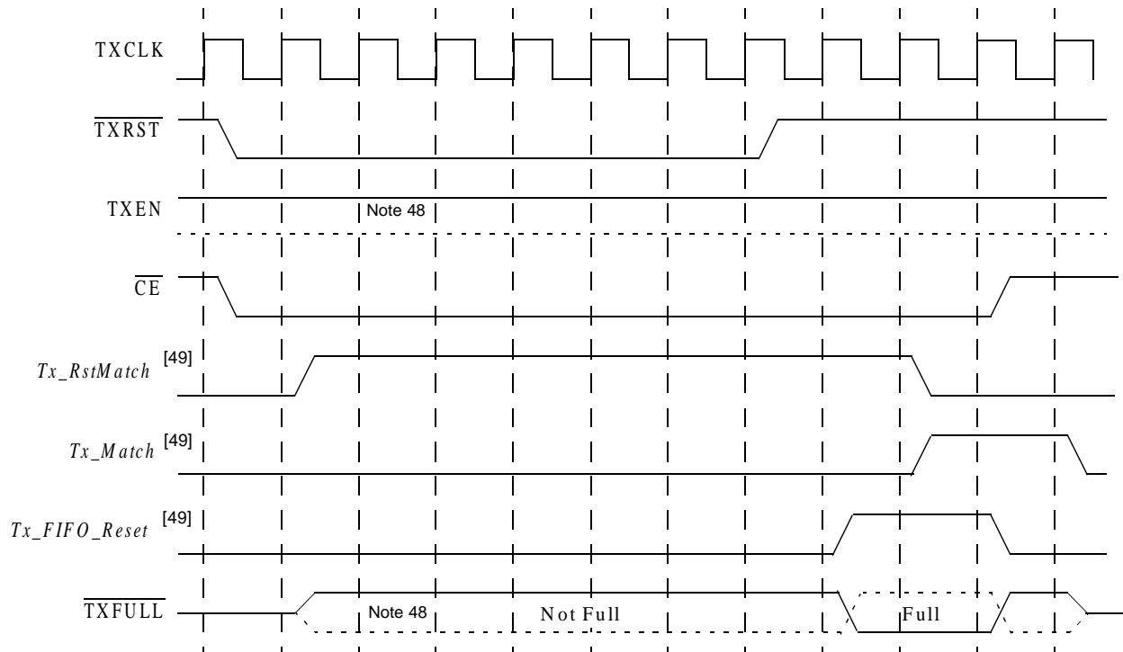
Figure 13. Transmit FIFO Reset Sequence
