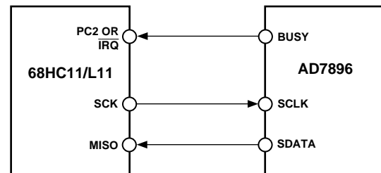
Figure 6. AD7896 to 68HC11/L11 Interface
