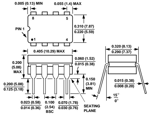
8-Lead Cerdip (Q-8)
