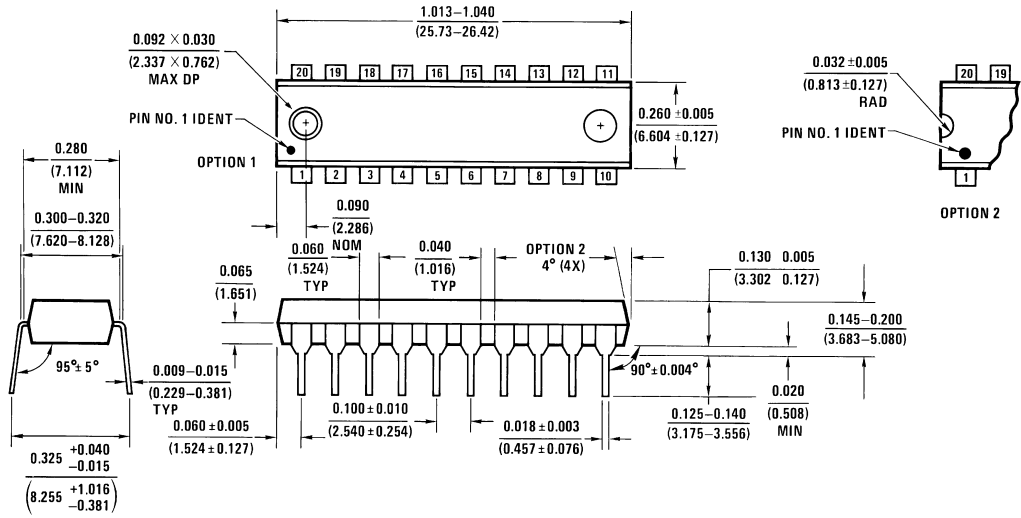
Dual-In-Line Plastic Package Order Number LM1972N NS Package Number N20A
