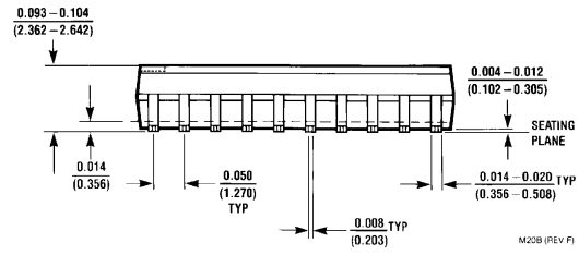
Surface Mount Package Order Number LM1972M NS Package Number M20B
