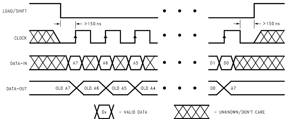
FIGURE 2. Timing Diagram
