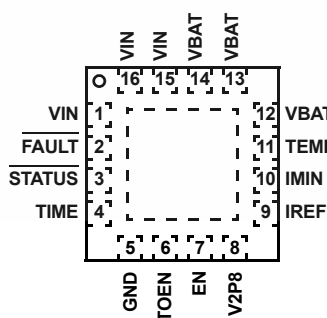
ISL6298 (16 LD QFN) TOP VIEW
