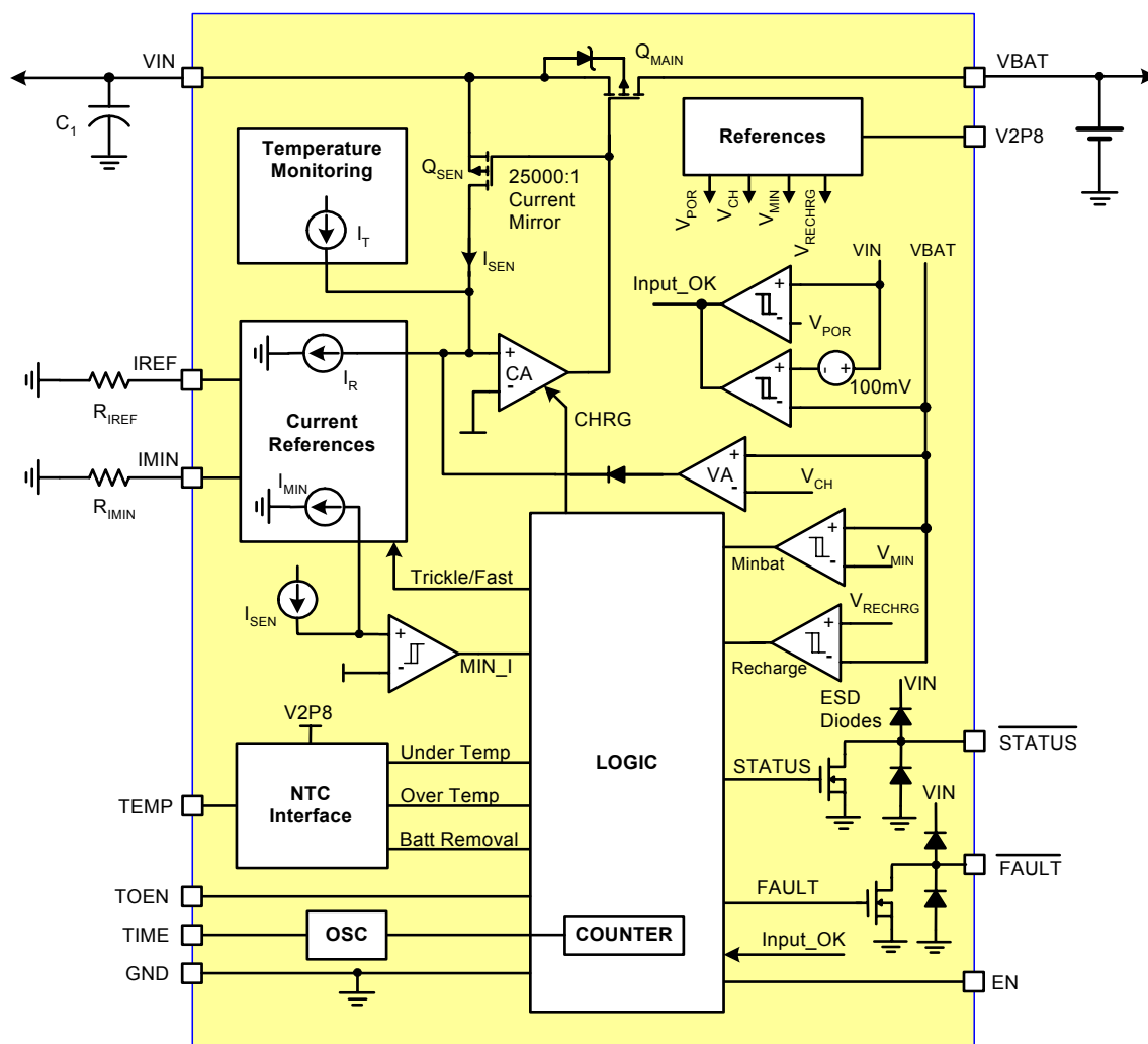
FIGURE 19. BLOCK PROGRAM
