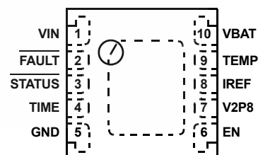
ISL6298 (10 LD DFN) TOP VIEW
