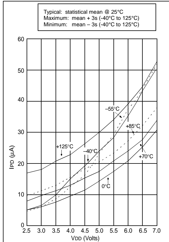
FIGURE 14-8: MAXIMUM IPD vs. VDD, WATCHDOG ENABLED
