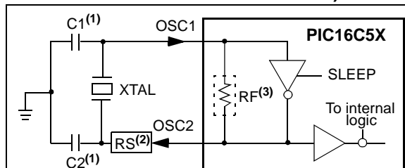
FIGURE 4-1: CRYSTAL/CERAMIC RESONATOR OPERATION (HS, XT OR LP OSC CONFIGURATION)
