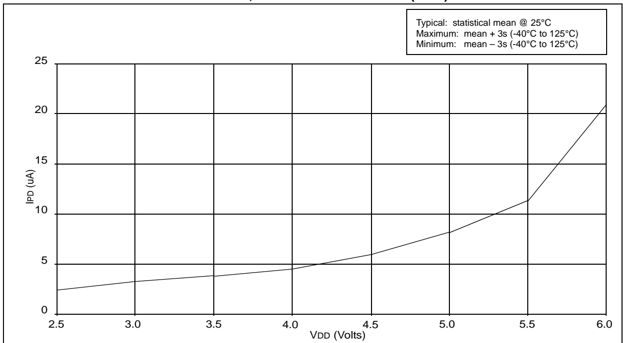
FIGURE 18-5: TYPICAL I PD vs. V DD , WATCHDOG DISABLED (25°C)
