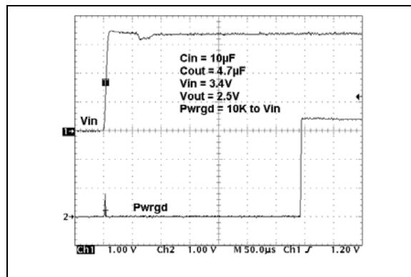
FIGURE 2-29: Power Good (PWRGD) Timing.
