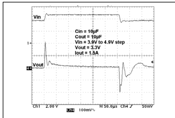
FIGURE 2-30: Dynamic Line Response (3.3V Fixed).
