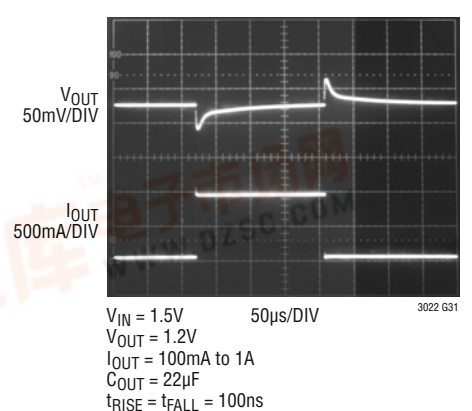
Transient Response
