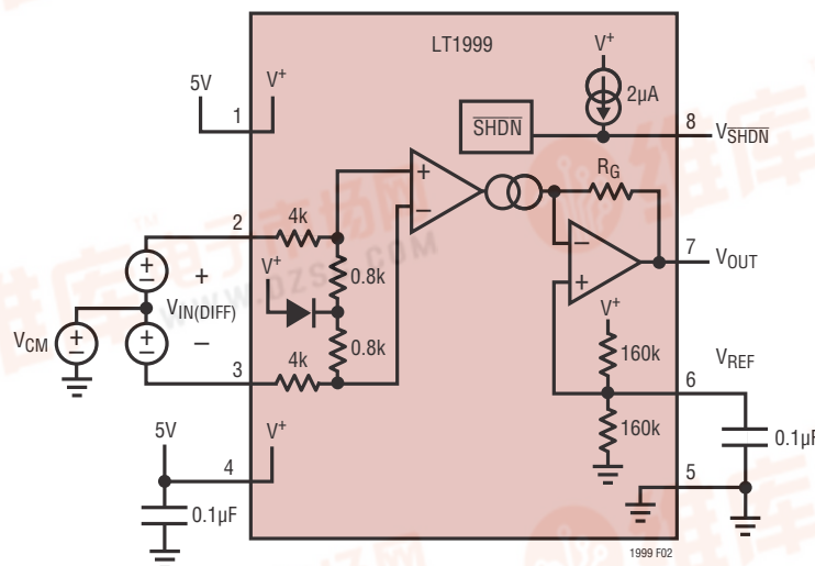
Figure 2. Test Circuit
