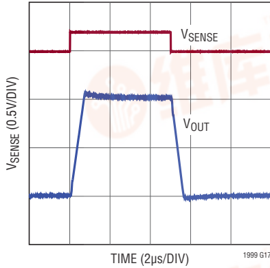
LT1999-10 Pulse Response
