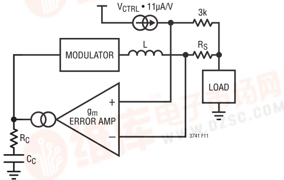
Figure 11. LT3741 Average Current Mode Control Scheme
