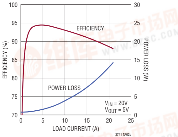
Efficiency and Power Loss vs Load Current
