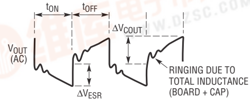
Figure 5. The Output Ripple Waveform of a Boost Converter
