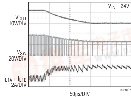
SEPIC FBX Frequency Foldback Waveforms During Overcurrent
