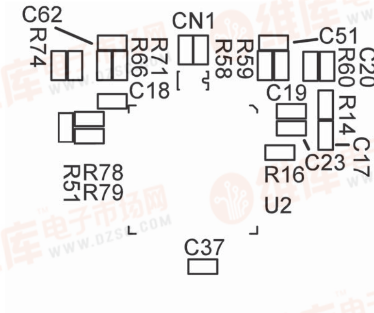
Silkscreen Top
