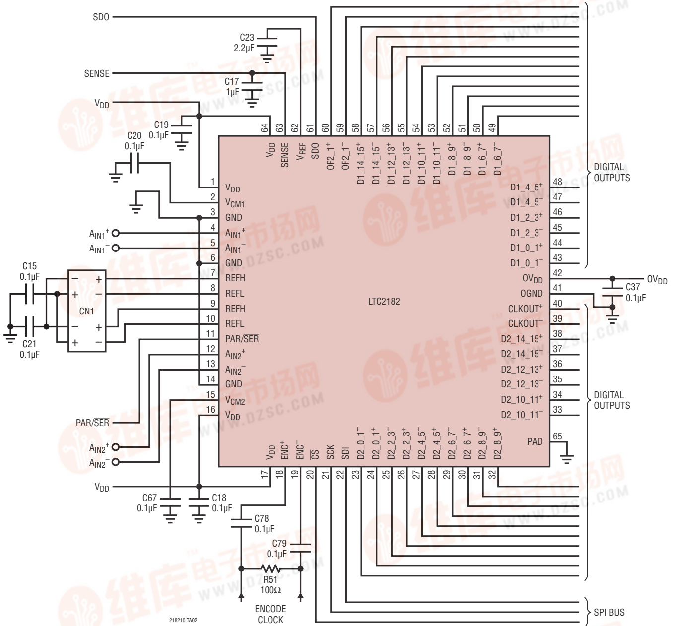
LTC2182 Schematic
