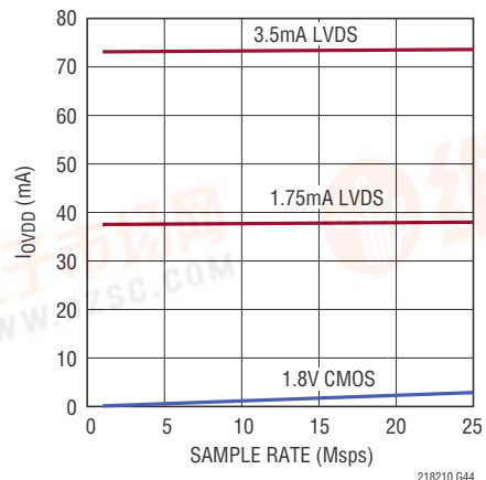
LTC2180: I_{OYDD} vs Sample Rate, 5\text{MHz} , -1\text{dBFS} , Sine Wave Input on Each Channel
