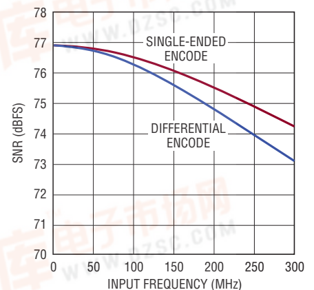
LTC2181: SNR vs Input Frequency, -1\text{dBFS} , 40\text{Mpsps} , 2\text{V} Range
