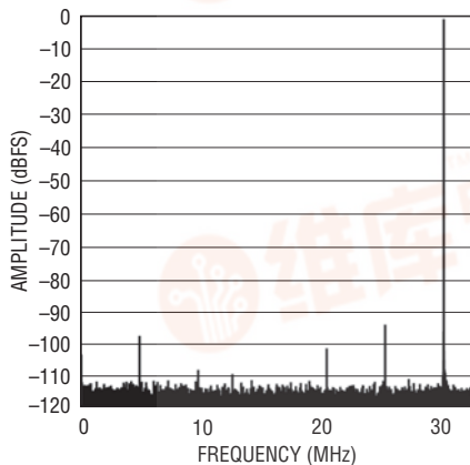
LTC2182: 64k Point FFT, f_{IN} = 30\text{MHz} , -1\text{dBFS} , 65Msps
