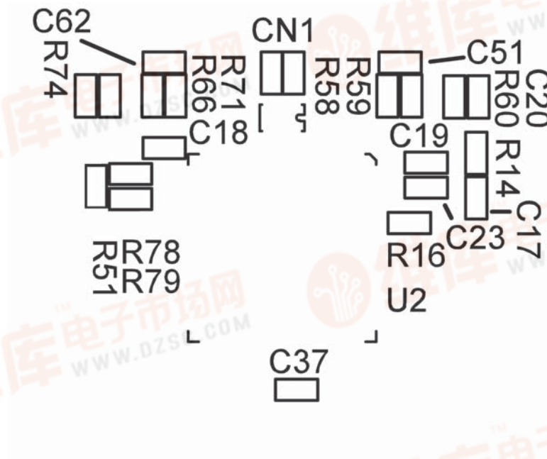
Silkscreen Top
