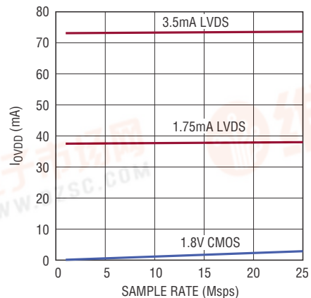
LTC2180: I_{OYDD} vs Sample Rate, 5\text{MHz} , -1\text{dBFS} , Sine Wave Input on Each Channel
