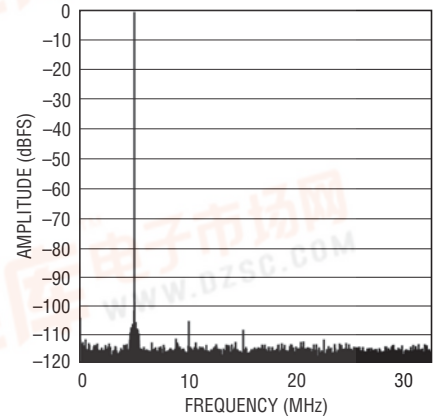
LTC2182: 64k Point FFT, f_{IN} = 5\text{MHz} , -1\text{dBFS} , 65Msps
