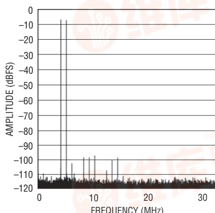
LTC2182: 64k Point 2-Tone FFT, f_{IN} = 69\text{MHz} , 70\text{MHz} , -7\text{dBFS} , 65Msps
