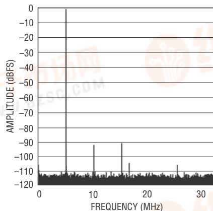
LTC2182: 64k Point FFT, f_{IN} = 70\text{MHz} , -1\text{dBFS} , 65Msps
