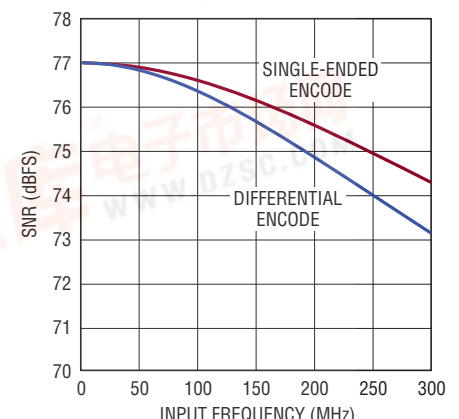
LTC2182: SNR vs Input Frequency, -1\text{dB} , 65Msps, 2V Range
