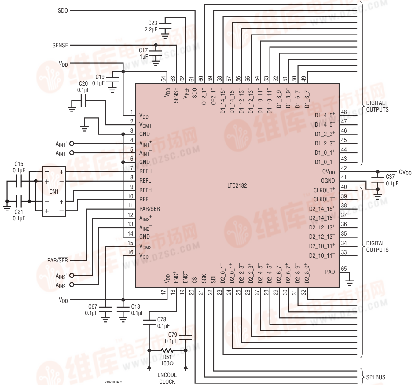
LTC2182 Schematic
