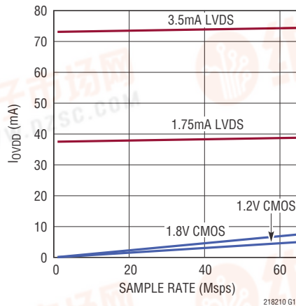
LTC2182: I_{QVDD} vs Sample Rate, 5MHz, -1dBFS, Sine Wave Input on Each Channel
