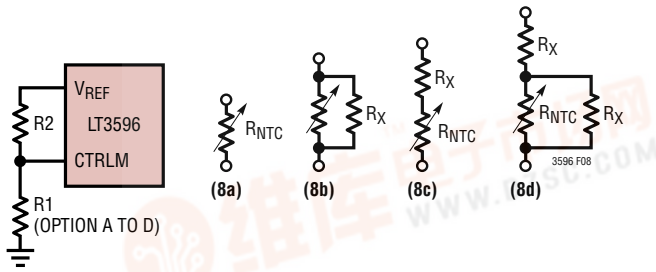
Figure 8. Programming the CTRLM Pin
