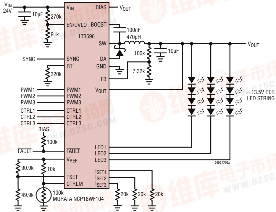
24V 200kHz Step-Down 4W, 100mA LED Driver
