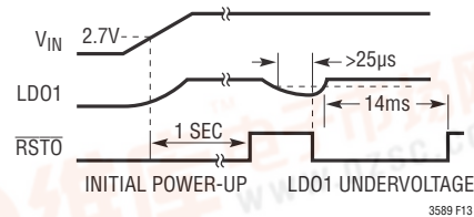
Figure 13. Initial Power-Up and LD01 Undervoltage \overline{\text{RSTO}} Timing
