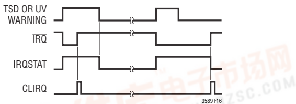
Figure 16. \overline{\text{IRQ}} and IRQSTAT Status Register Warning Timing
