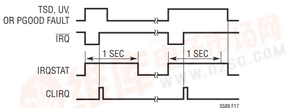
Figure 17. \overline{\text{IRQ}} and IRQSTAT Status Register Fault Timing
