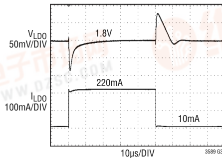
LD02, LD03, LD04 Load Step Response
