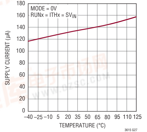
No Load Supply Current vs Temperature
