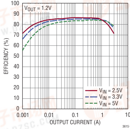
Efficiency vs Load Current ( V_{MODE} = 0V )
