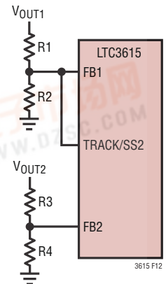
Figure 12. Set-Up for Ratiometric Tracking
