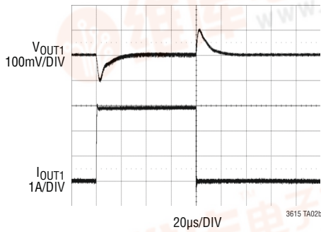
V OUT1 Waveform
