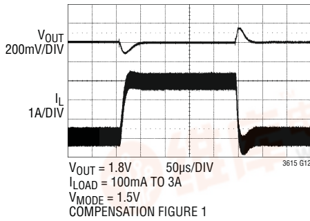
Load Step Transient in FCM External Compensation
