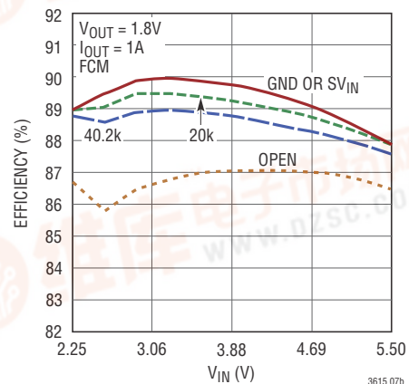
(7b) Efficiency vs SRLIM Resistor Programming
