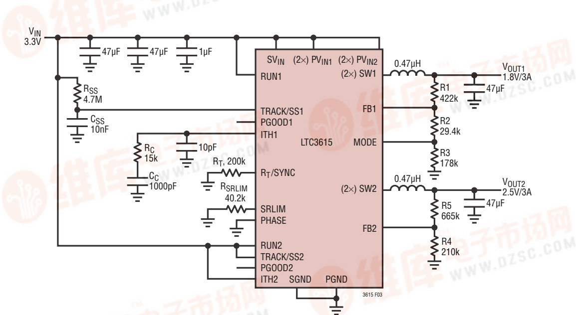
Figure 3. Soft-Start and Compensation for Channel 1 Externally Programmed, Soft-Start and Compensation for Channel 2 Internally Programmed
