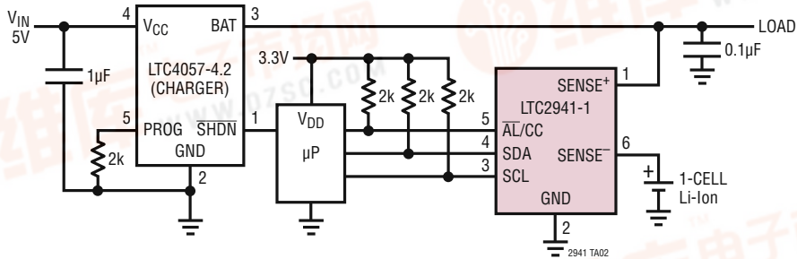
Single Cell Lithium-Ion Coulomb Counter with Battery Charger for Discharge Currents of up to 1A
