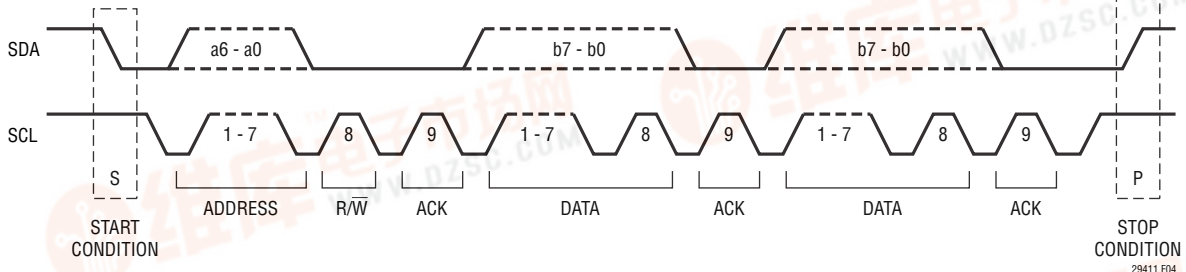
Figure 4. Data Transfer Over I 2 C or SMBus
