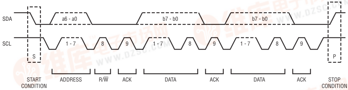
Figure 6. Data Transfer Over I²C or SMBus
