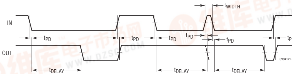
Figure 4. Falling-Edge Delayed Timing Diagram (LTC6994-1, POL = 1)
