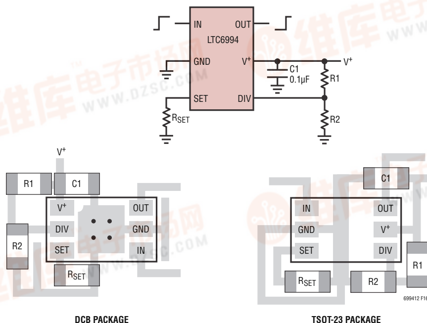
Figure 16. Supply Bypassing and PCB Layout
