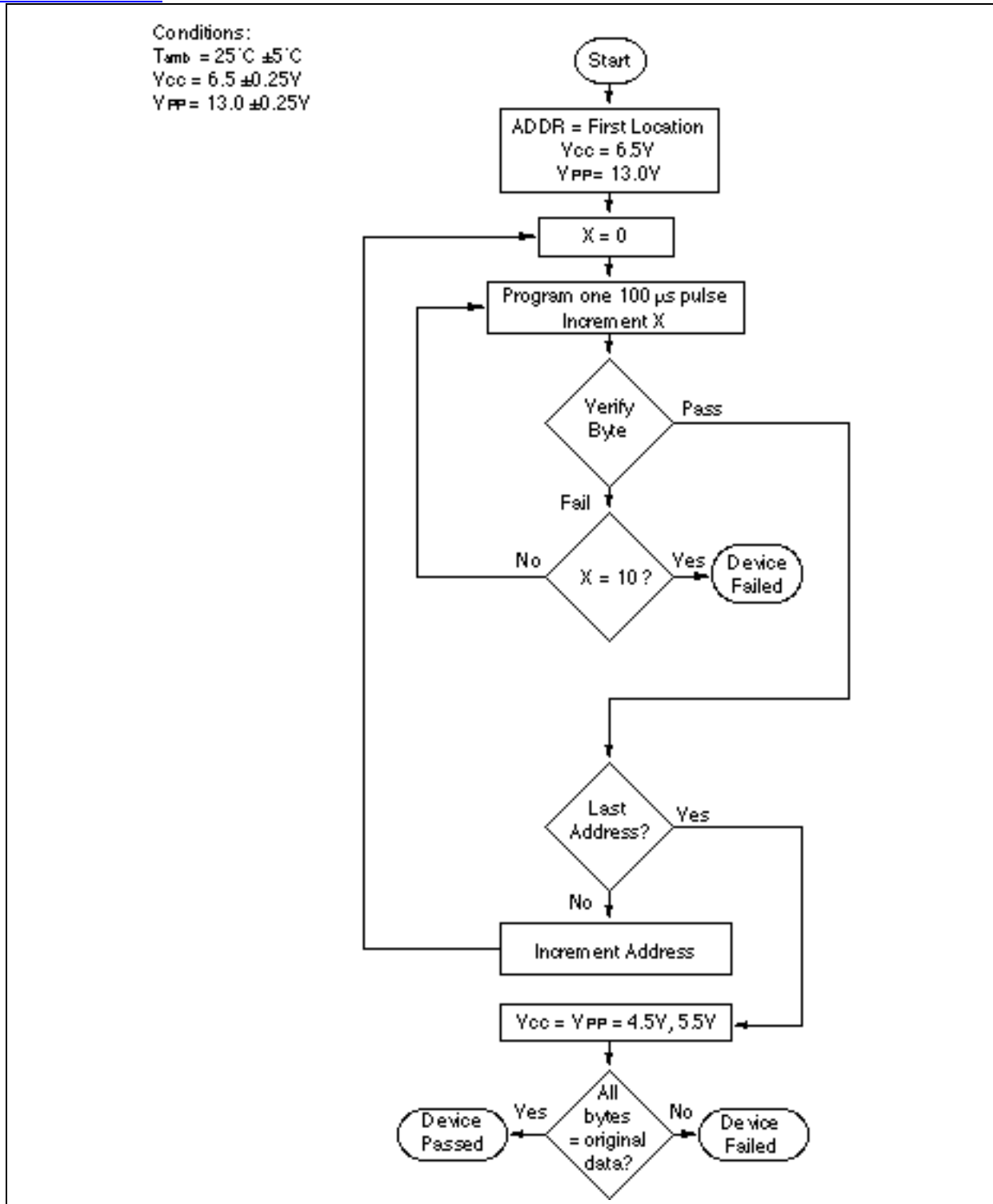
查询970198供应商 FIGURE 1-3 PROGRAMMING EXPRESS ALGORITHM
