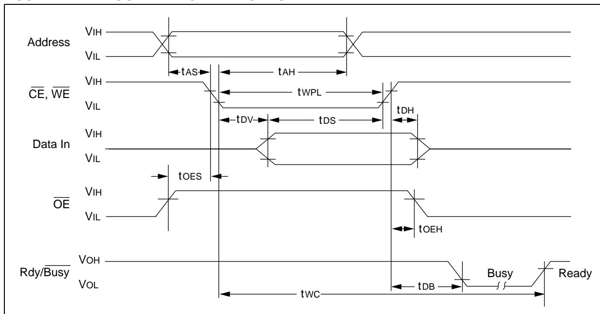
FIGURE 1-2: PROGRAMMING WAVEFORMS
