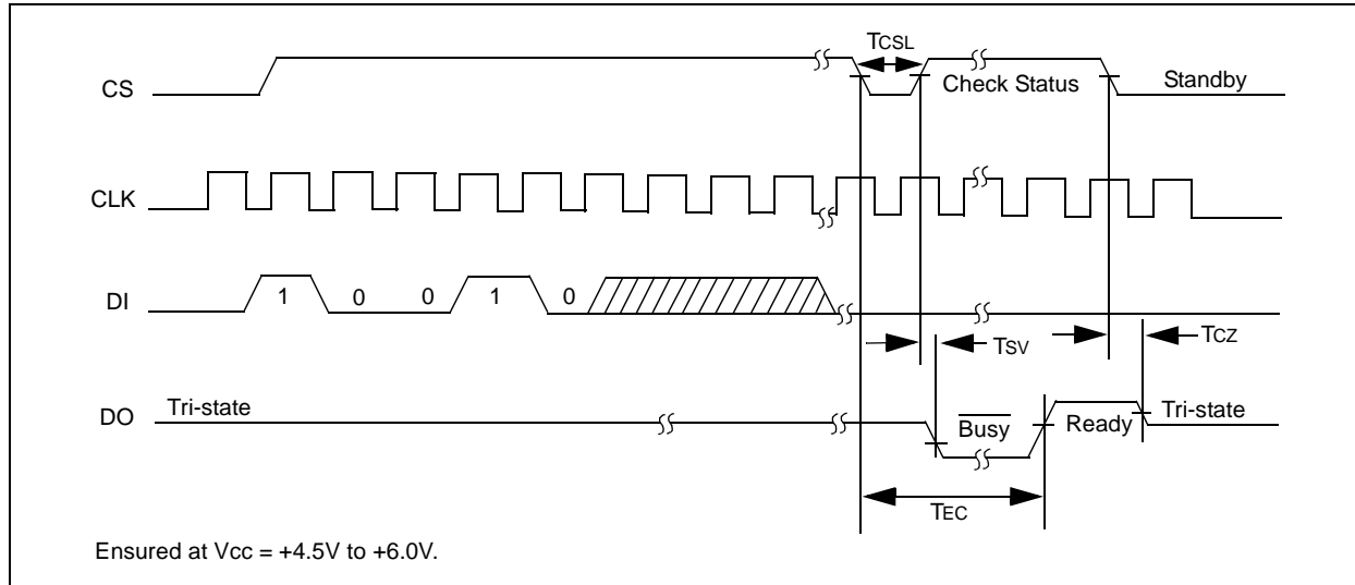
FIGURE 2-8: SERIAL TIMING
