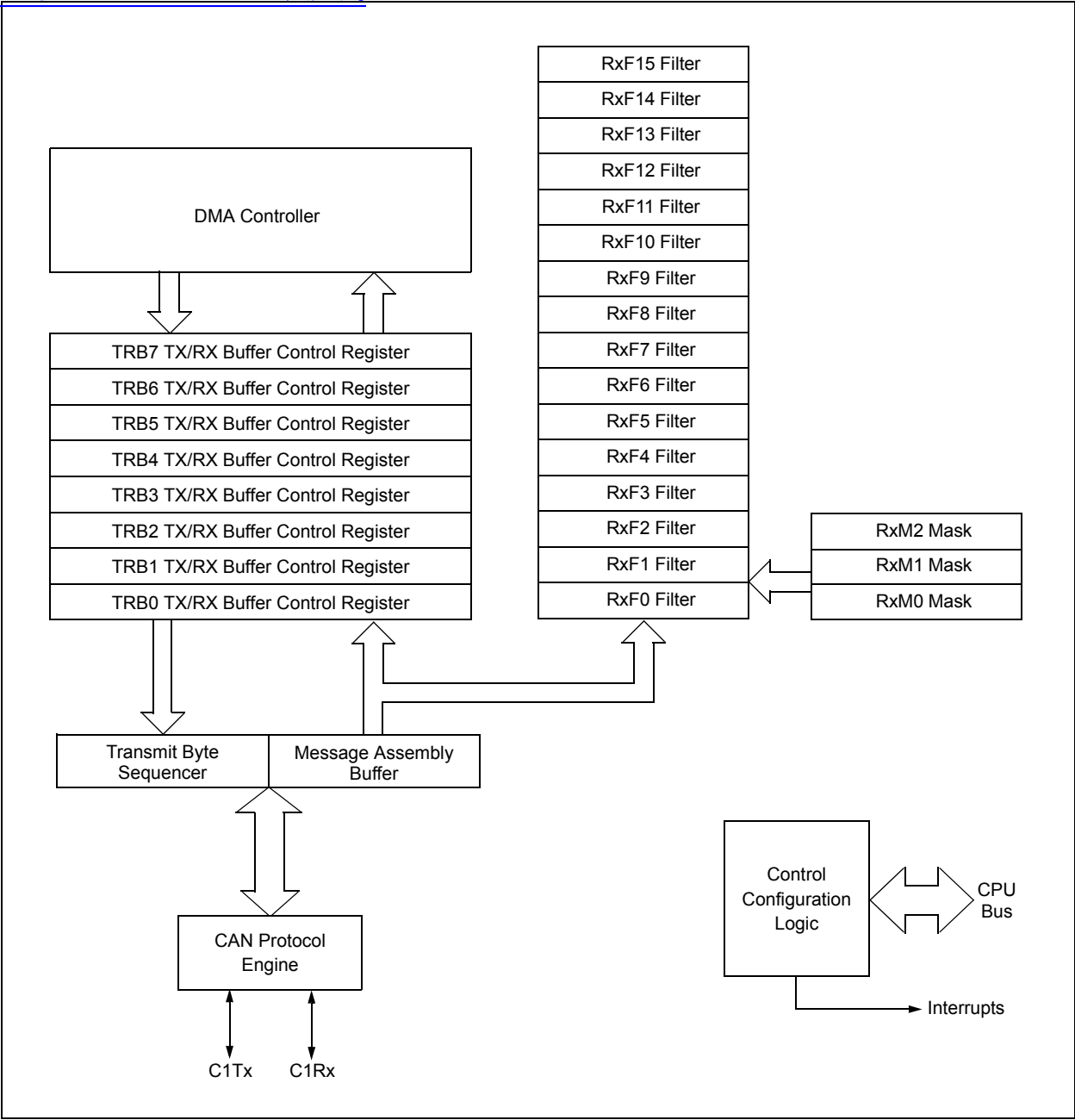
FIGURE 20-36 dsPIC33FJ128MCX02/X04 CAN MODULE BLOCK DIAGRAM
