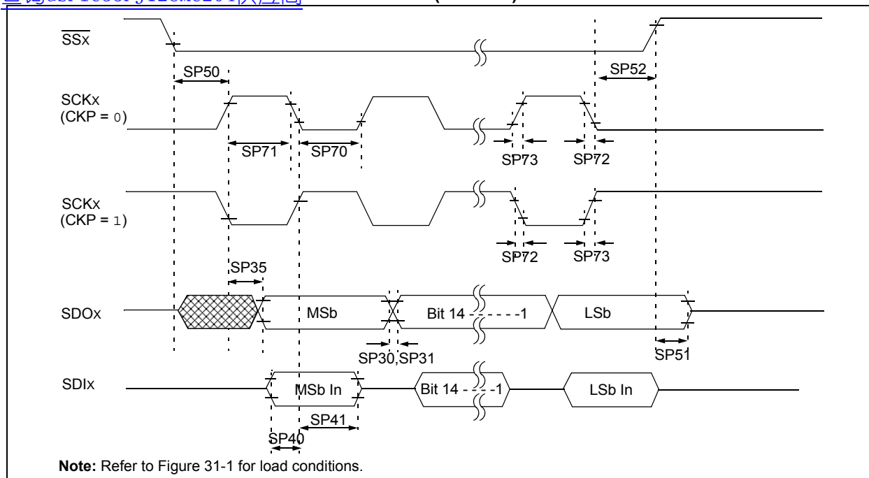
FIGURE 31-36: SPIx MODULE SLAVE MODE (CKE = 0) TIMING CHARACTERISTICS
