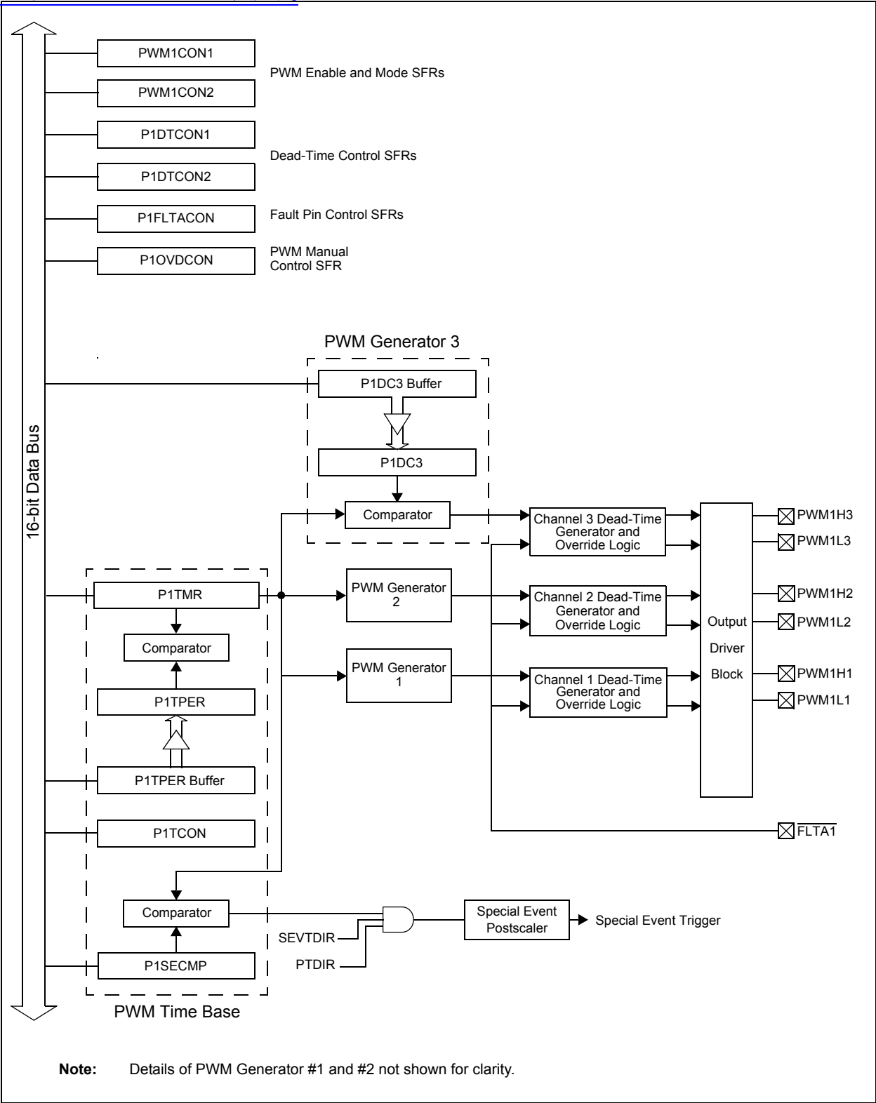
FIGURE 16-3: 3-COMPONENT PWM MODULE BLOCK DIAGRAM (PWM1)
