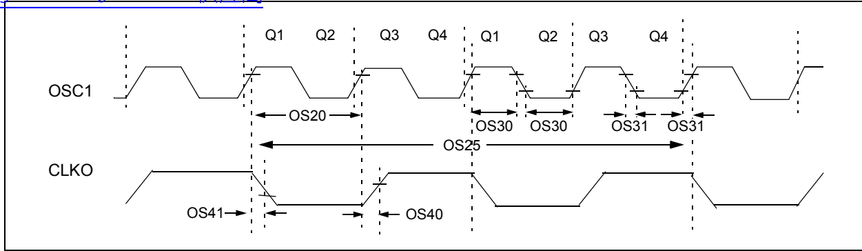
FIGURE 31-12: EXTERNAL CLOCK TIMING
