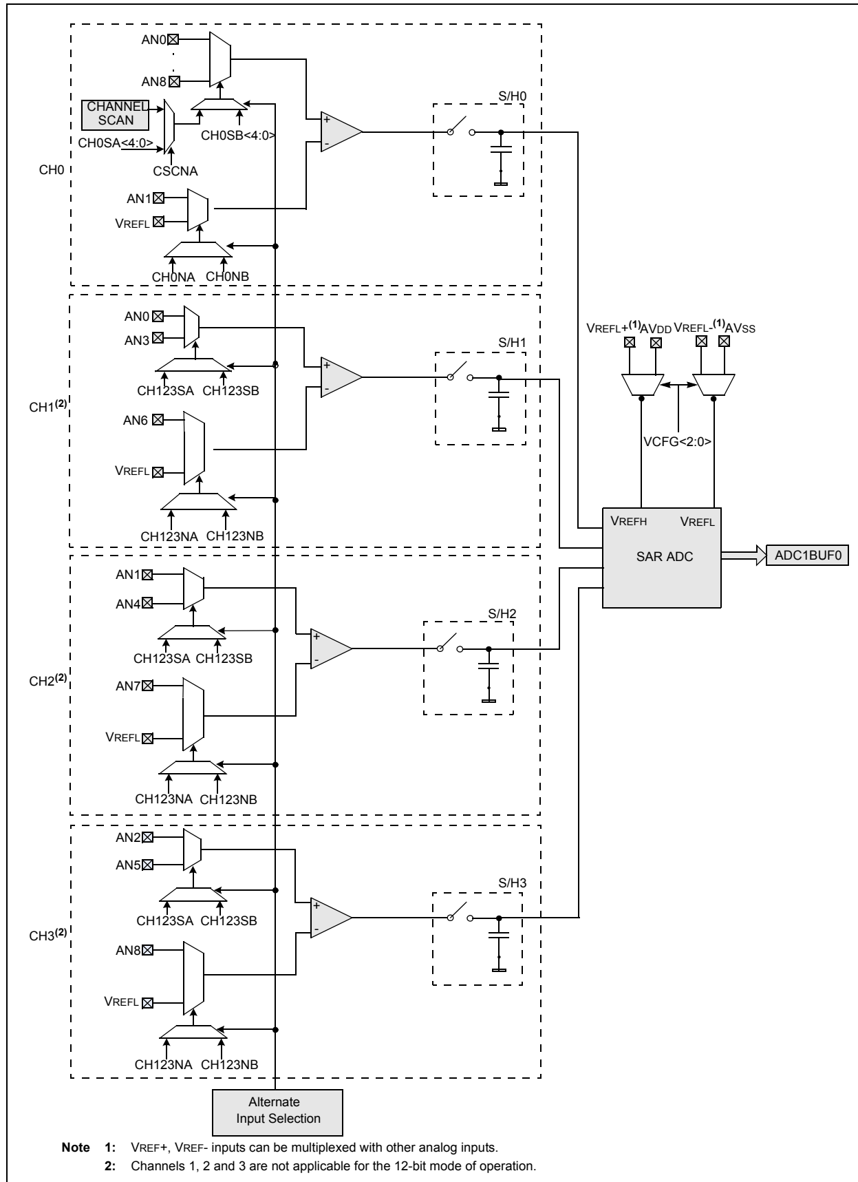
FIGURE 22-1 dsPIC33FJ128MC204/804 BLOCK DIAGRAM FOR dsPIC33FJ32MC304, dsPIC33FJ64MC204/804 AND dsPIC33FJ128MC204/804 DEVICES
