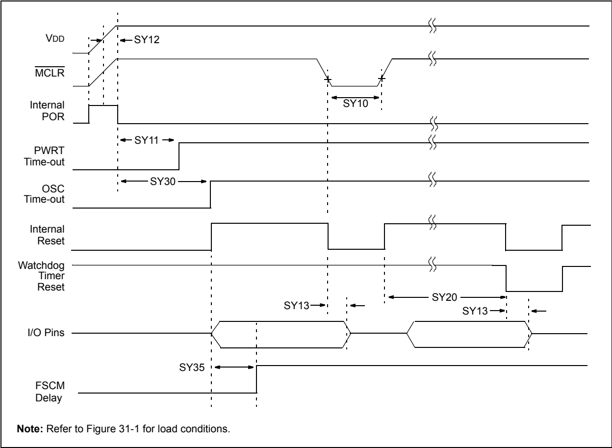
FIGURE 31-4: dsPIC33FJ128MCX02/X04 RESET, WATCHDOG TIMER, OSCILLATOR START-UP TIMER AND POWER-UP TIMER TIMING CHARACTERISTICS
