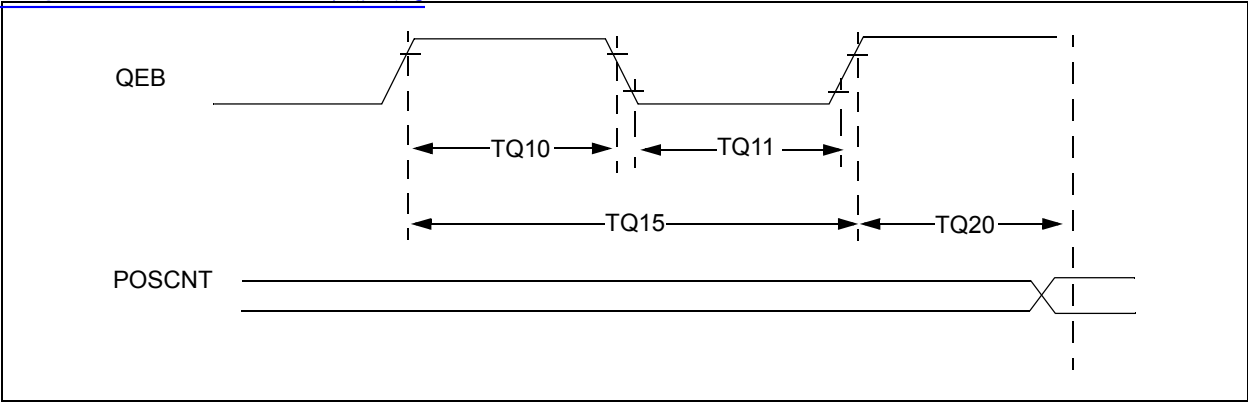
FIGURE 31-6: dsPIC33FJ128MCX02/X04 (QEI MODULE) EXTERNAL CLOCK TIMING CHARACTERISTICS
