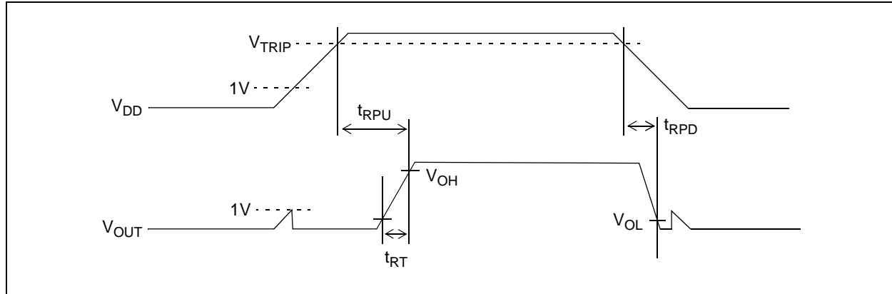
FIGURE 1-1: Timing Diagram.
