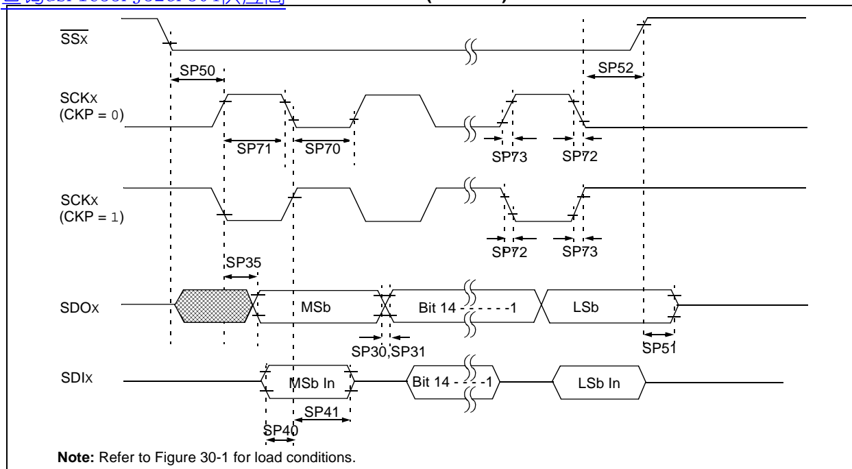
FIGURE 30-30: SPIx MODULE SLAVE MODE (CKE = 0) TIMING CHARACTERISTICS
