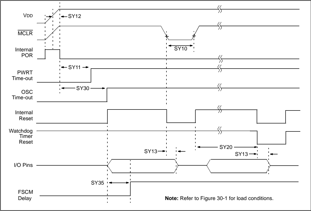
FIGURE 30-4: dsPIC33FJ32GP302/304 响应高 RESET, WATCHDOG TIMER, OSCILLATOR START-UP TIMER AND POWER-UP TIMER TIMING CHARACTERISTICS
