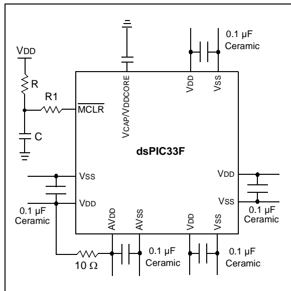
FIGURE 2-1: dsPIC33FJ32GP302/304 (RECOMMENDED) MINIMUM CONNECTION
