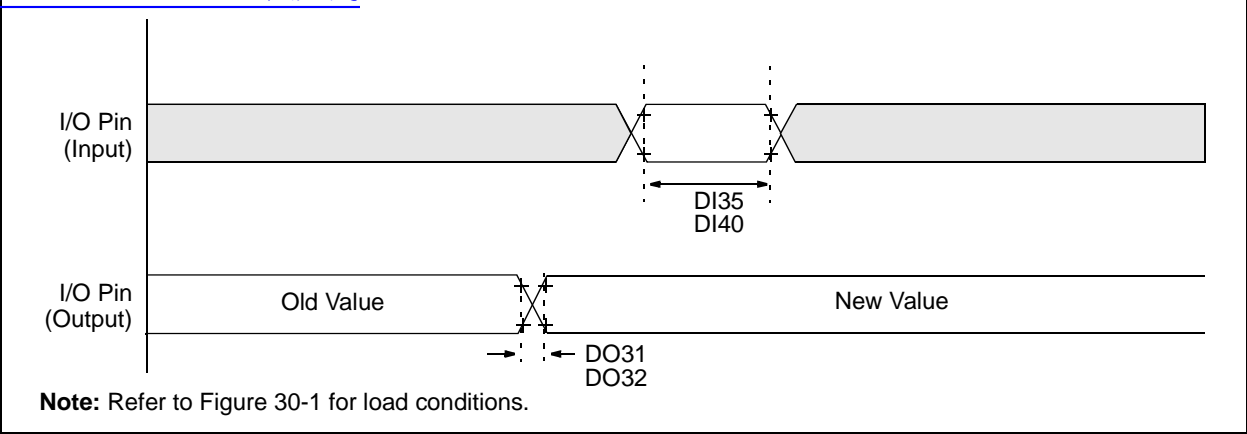
FIGURE 30-13: CLKO AND I/O TIMING CHARACTERISTICS
