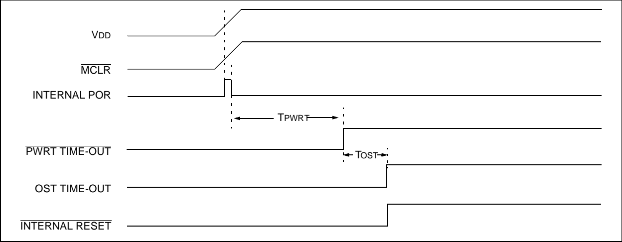
FIGURE 10-10: TIME-OUT SEQUENCE ON POWER-UP ( \overline{\text{MCLR}} TIED TO \text{V}_{\text{DD}} )
