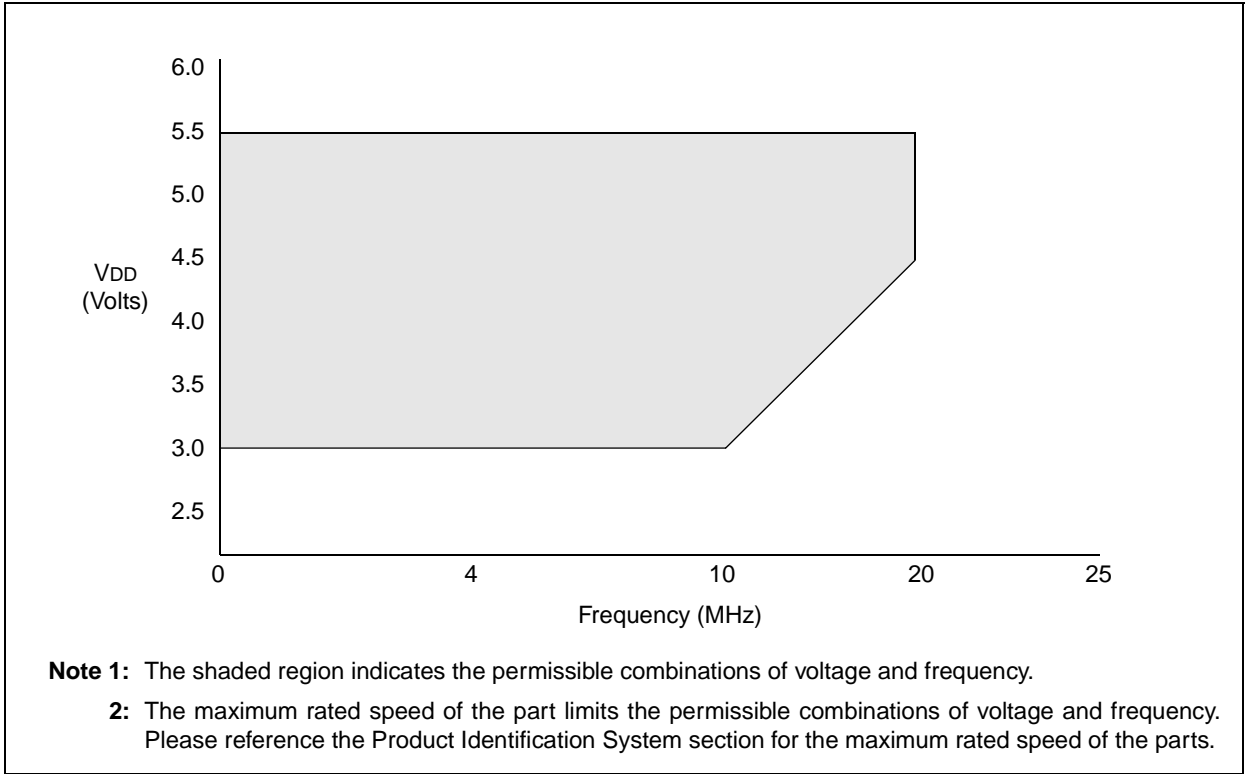
FIGURE 13-2: PIC16CE62X VOLTAGE-FREQUENCY GRAPH, -40°C ≤ TA < 0°C, +70°C < TA ≤ +125°C
