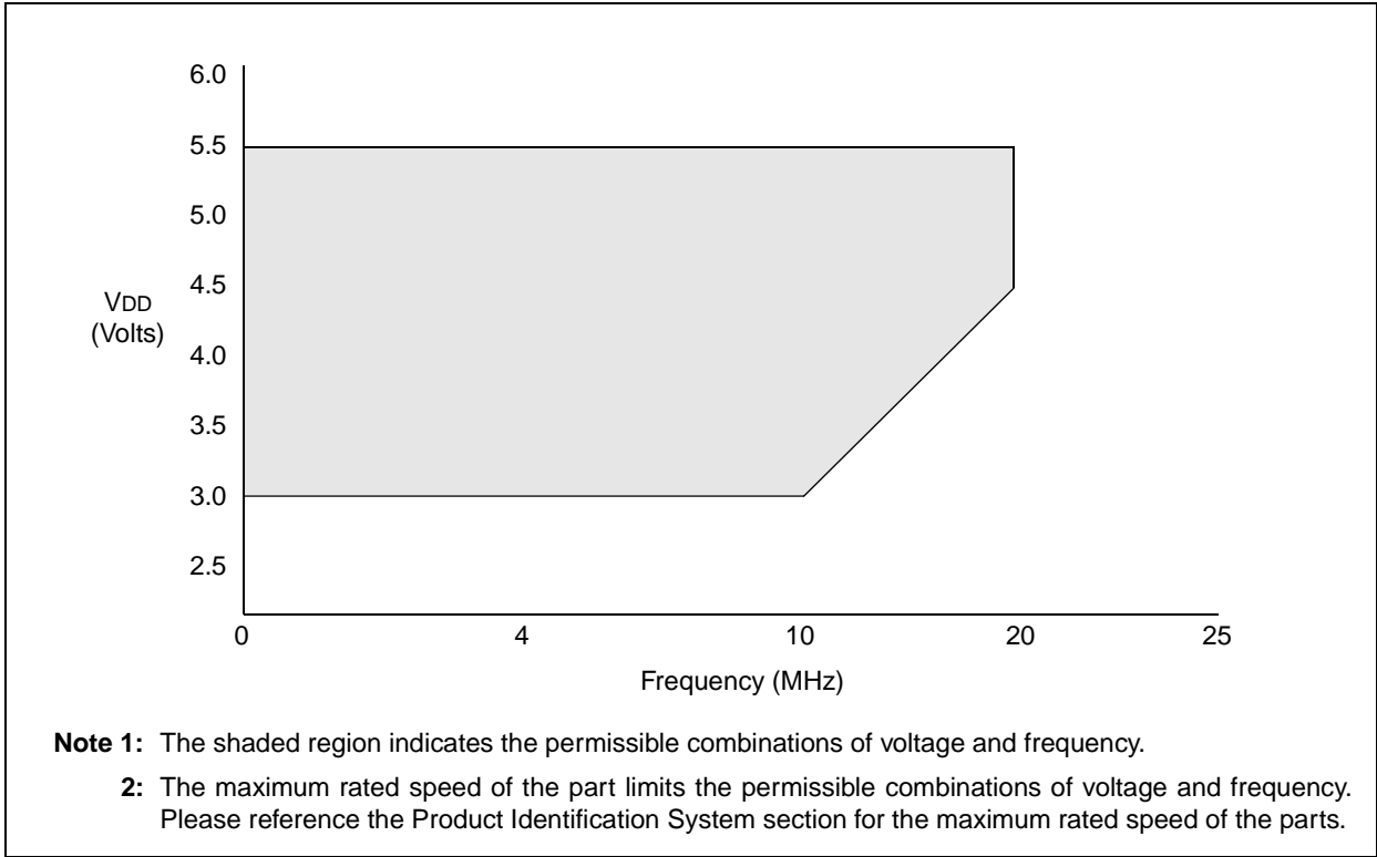
FIGURE 13-2: PIC16CE62X VOLTAGE-FREQUENCY GRAPH, -40°C ≤ TA < 0°C, +70°C < TA ≤ +125°C
