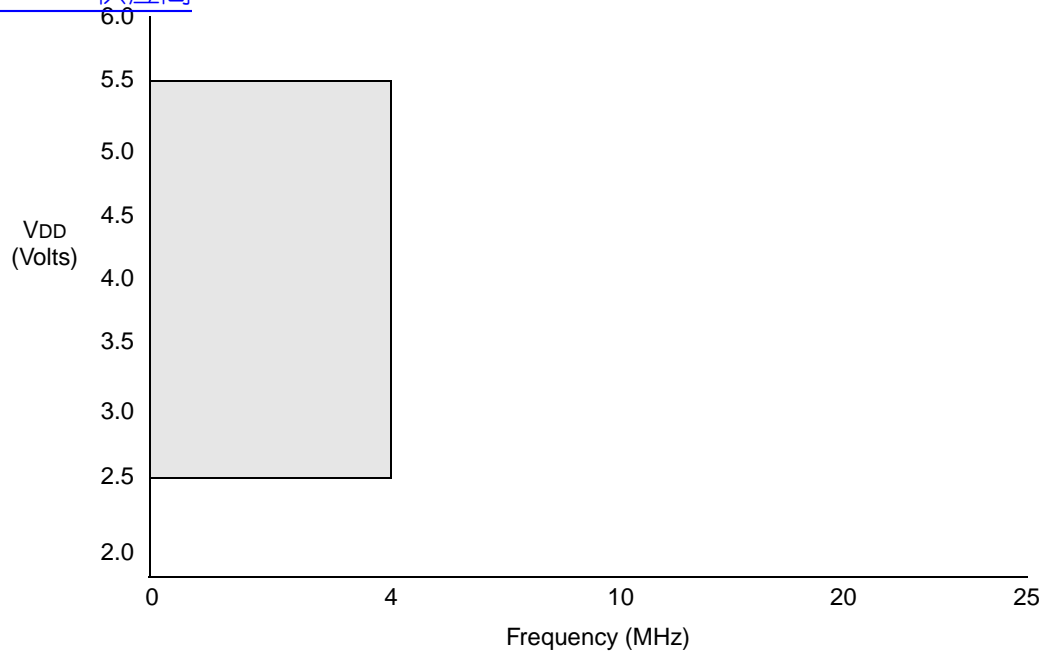
FIGURE 13-3: PIC16LCE62X VOLTAGE-FREQUENCY GRAPH, -40^{\circ}\text{C} \leq T_A < +125^{\circ}\text{C}
