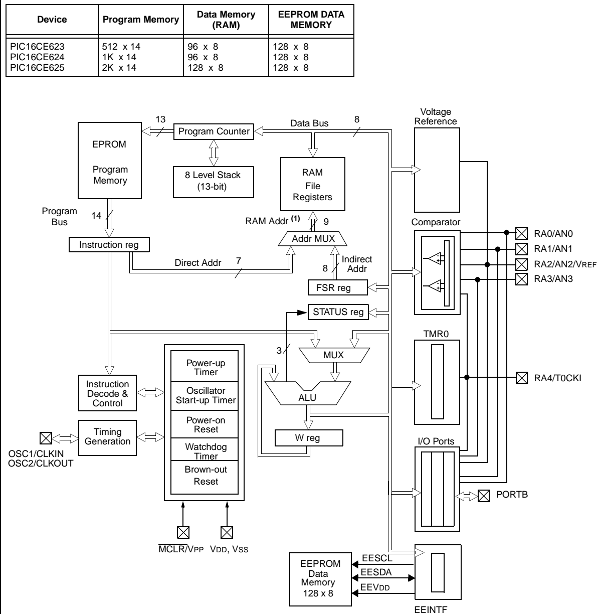
FIGURE 3-1. BLOCK DIAGRAM
