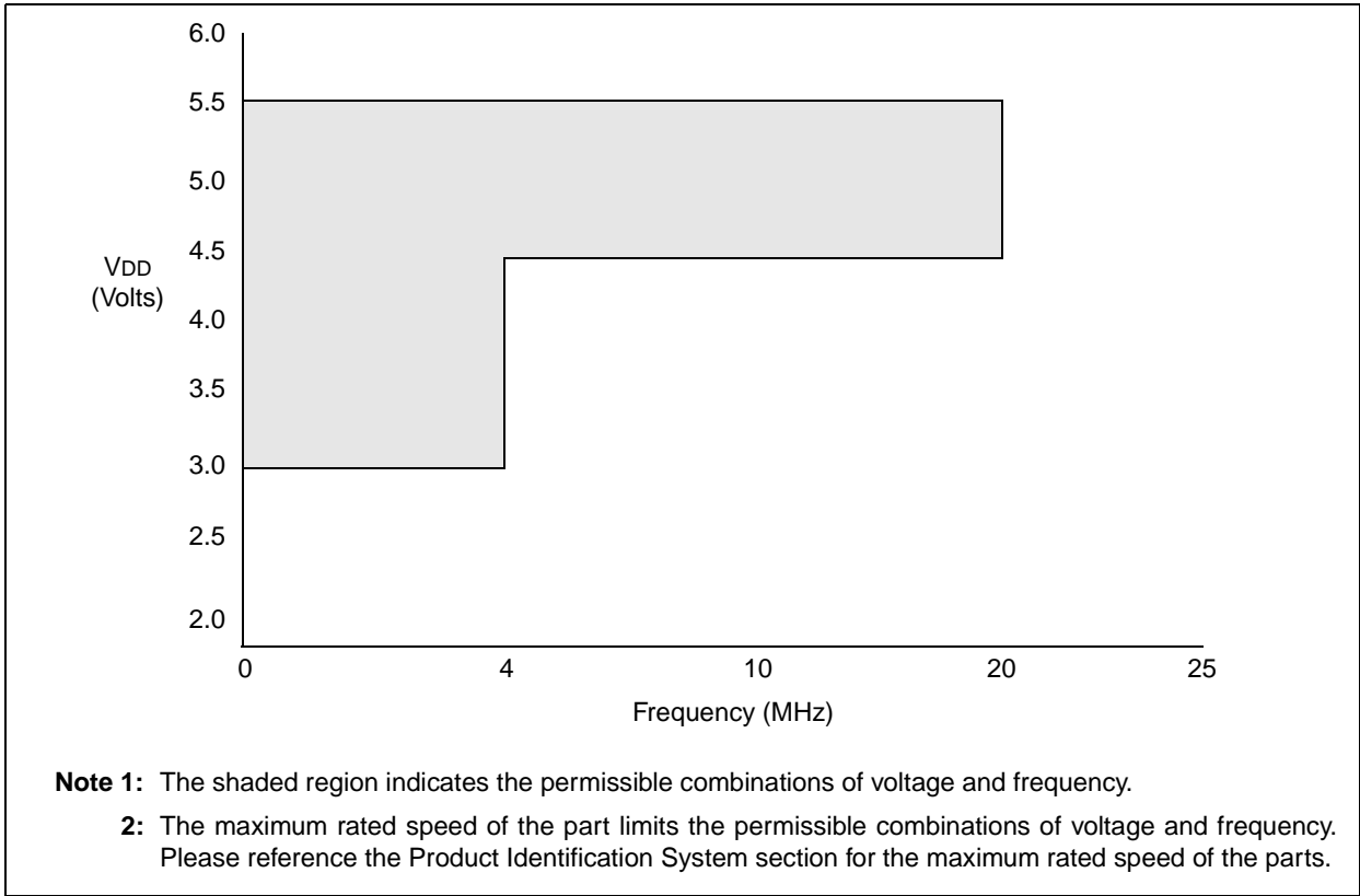
FIGURE 13-2: PIC16CE62X VOLTAGE-FREQUENCY GRAPH, -40°C ≤ TA < 0°C, +70°C < TA ≤ +125°C
