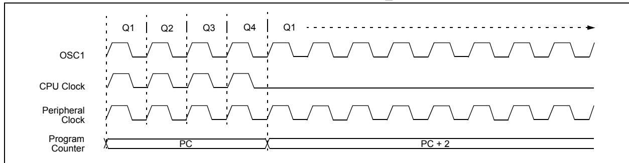
FIGURE 4-7: TRANSITION TIMING FOR ENTRY TO PRI_IDLE MODE
