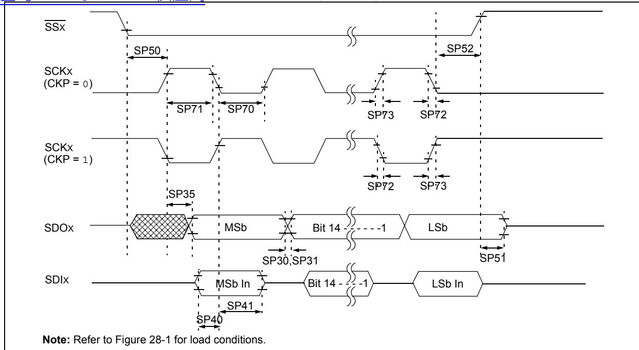
FIGURE 28-31: SPIx MODULE SLAVE MODE (CKE = 0) TIMING CHARACTERISTICS
