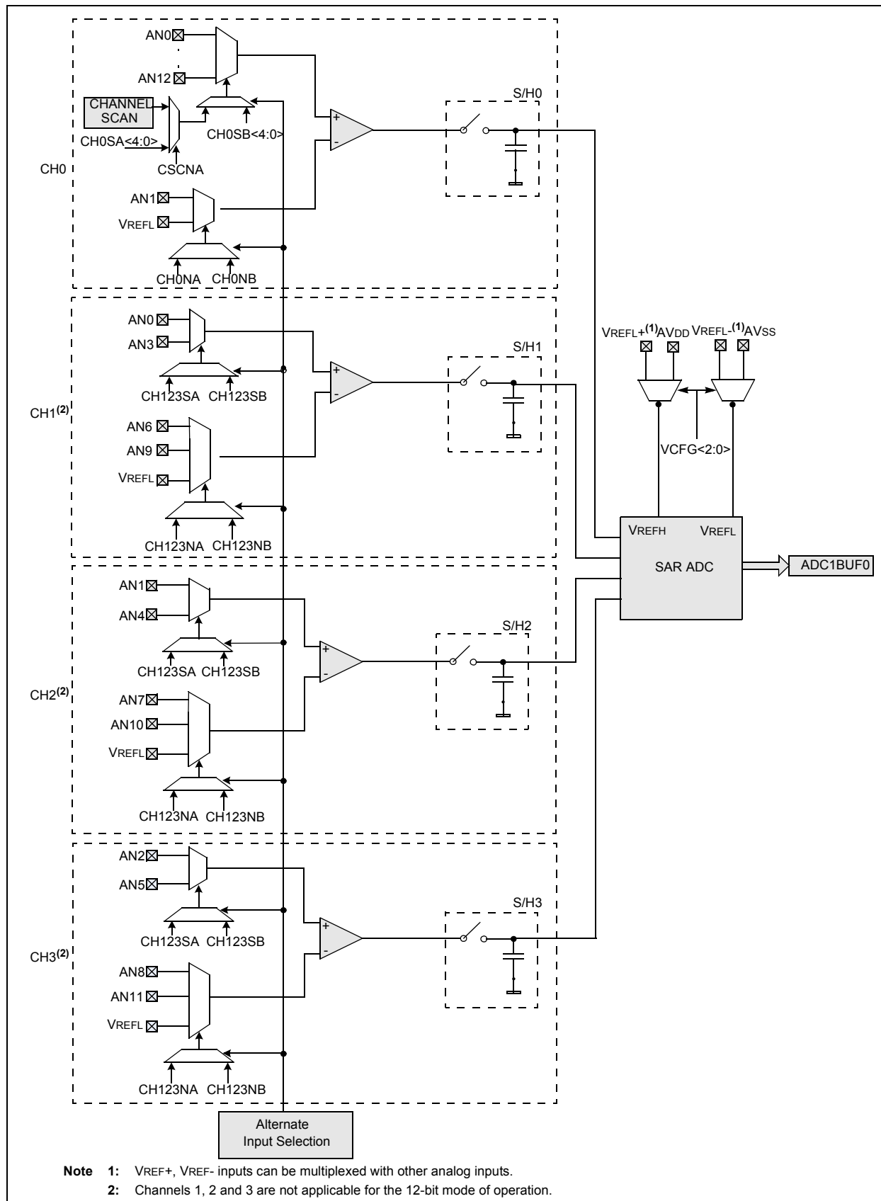
FIGURE 20-1: 128GPX02/X04 ADC1 MODULE BLOCK DIAGRAM FOR PIC24HJ32GP304, PIC24HJ64GP204/504 AND PIC24HJ128GP204/504 DEVICES
