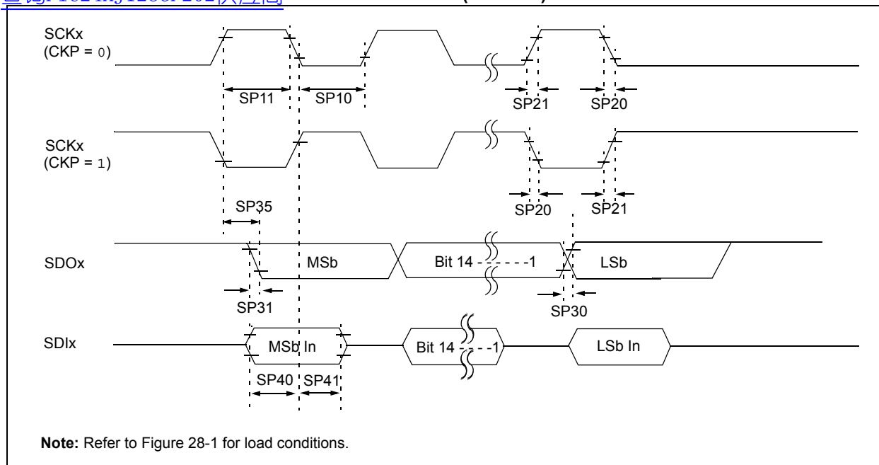
FIGURE 28-19: SPIx MASTER MODE (CKE = 0) TIMING CHARACTERISTICS
