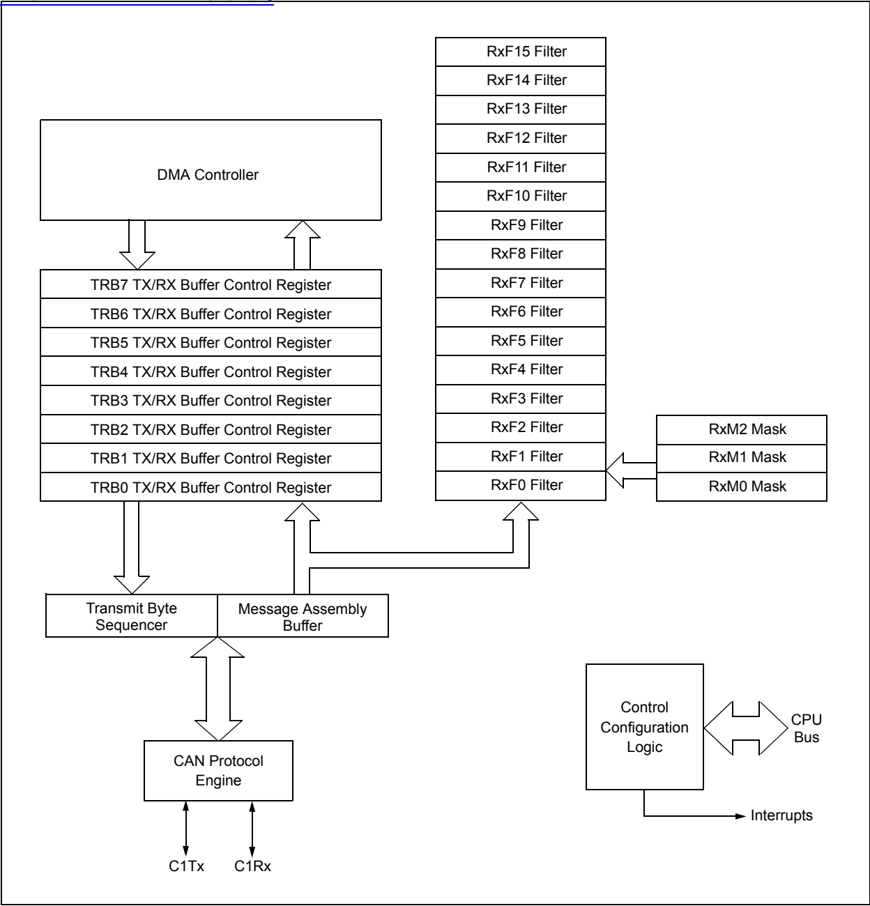
FIGURE 19-1: 128GPX02/X04 CAN™ MODULE BLOCK DIAGRAM
