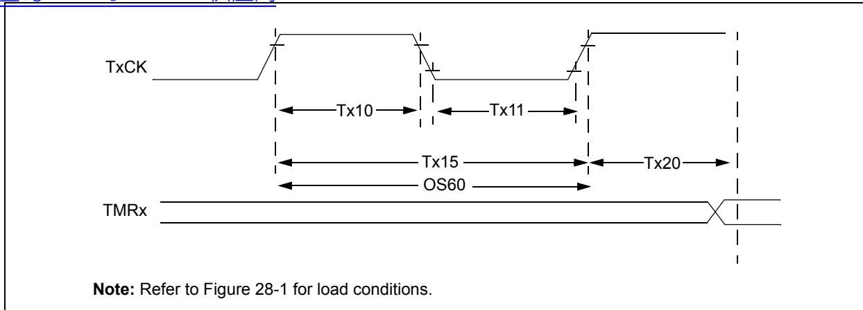
FIGURE 28-5: PIC24HJ128GPX02/X04 AND 4 EXTERNAL CLOCK TIMING CHARACTERISTICS
