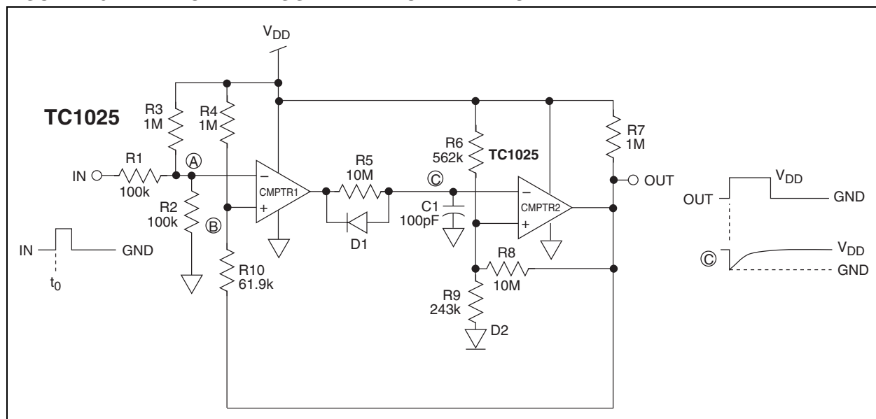
FIGURE 4-3: NON-RETRIGGERABLE MULTIVIBRATOR
