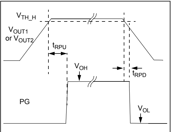
FIGURE 4-1: Power-Good Timing.
