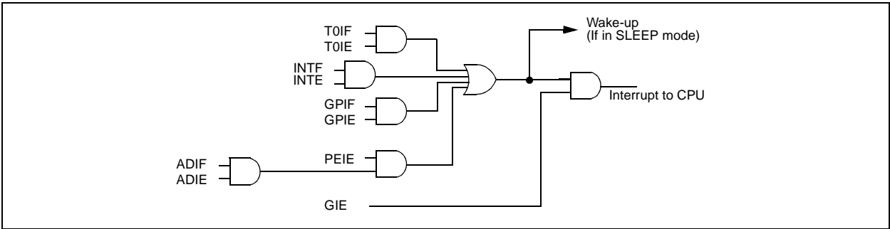
FIGURE 9-13: INTERRUPT LOGIC
