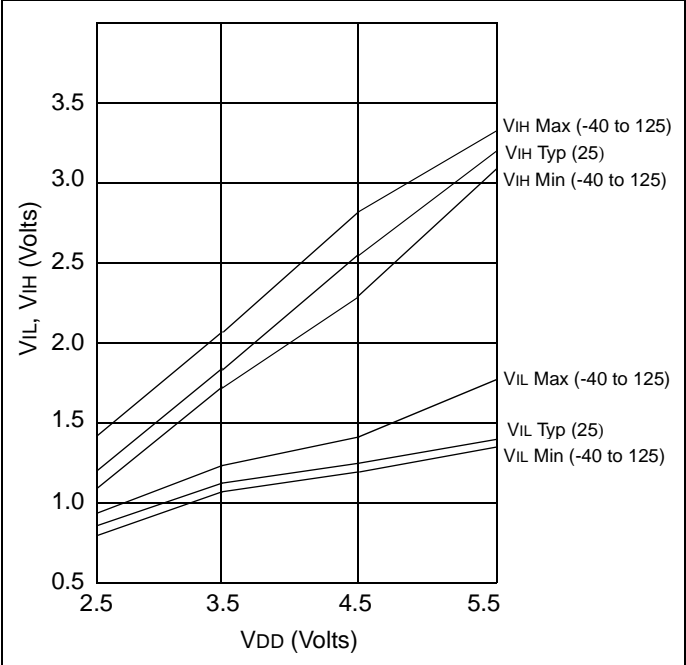
查询PIC12C67X供应商 FIGURE 13-1: V_{IL} , V_{IH} OF NMCLR AND T0CKI vs. V_{DD}
