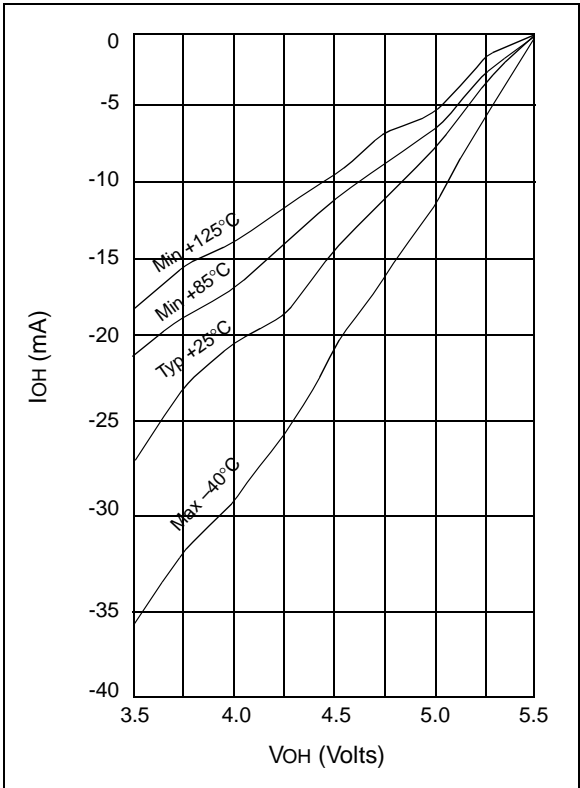
FIGURE 13-6: I_{OH} vs. V_{OH} , V_{DD} = 5.5\text{ V}
