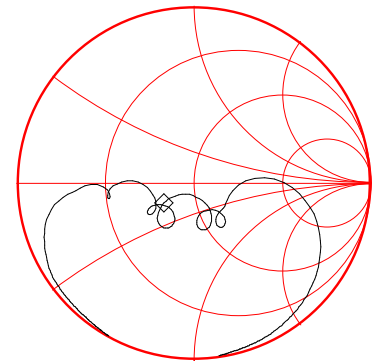
S11 Smith Chart
