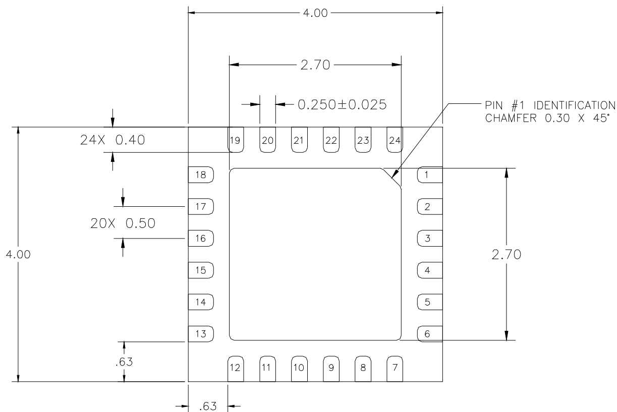
BOTTOM VIEW
